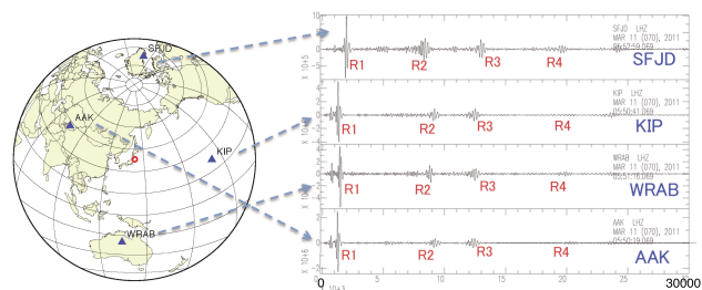
Fig. 2. Multi-orbit long-period surface waves for the 2011 off the Pacific coast of Tohoku Earthquake. Waveforms are vertical component with a bandpass filter from 3 to 10 mHz. Amplitudes decay systematically in time at stations in any directions from the source, representing a point-like source.
