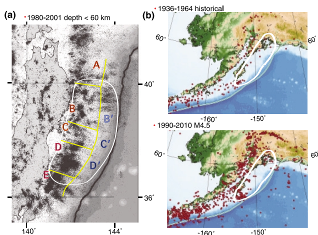
Fig. 1. Seismicity in subduction zones of (a) Tohoku, eastern Japan, and (b) Alaska with fault areas of the 2011 and 1964 earthquakes in white, compiled by Tohoku University (after Uchida et al. (2009)) and the U.S. Geological Survey, respectively. In eastern Japan, earthquakes in 1980–2001 at depths shallower than 60 km are plotted. The segmentation of seismogenic zones are shown in (a), following the national project of disaster prevention of Japan ( http://www.j-shis.bosai.go.jp/?lang=en ). In Alaska, earthquakes before the 1964 earthquake of magnitude over 5.0 are plotted from 1935 to 1964 and magnitude over 4.5 from 1990 to 2010.
