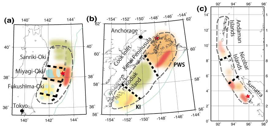
Fig. 3. Comparison of schematic views of source processes and related seismic activities for the (a) 2011 Tohoku, (b) 1964 Alaska, and (c) 2004 Sumatra earthquakes. Epicenters are shown by red stars, areas of major seismic moment release by orange patches and possible tsunami-excitation areas by red patches. In (a), the thick dashed lines represent the segments similar to Fig. 1(a), slow earthquakes including the 1896 great tsunami earthquake close to the trench are shown by four green patches, recent large Miyagi-Oki earthquakes in 1938 by light blue circles with a region of large excitation of high-frequency waves (Honda et al. , 2011) and many aftershocks in light yellow. In (b), the orange patch is called the Prince William Sound asperity (PWS), two blue circles near the Kodiak Island represent intraplate earthquakes in 1999 and 2001 with the Kodiak Island asperity (KI) in yellow, and a creeping segment between them is shown in green (Ratchkovski and Hansen, 2001; Freymueller et al. , 2008). In (c), the areas of large slips are estimated by teleseismic body waves in orange (Ammon et al. , 2005) and those estimated by tsunami waveforms in red (Tanioka et al. , 2006) with the three along-strike segments proposed by Lay et al. (2005).
