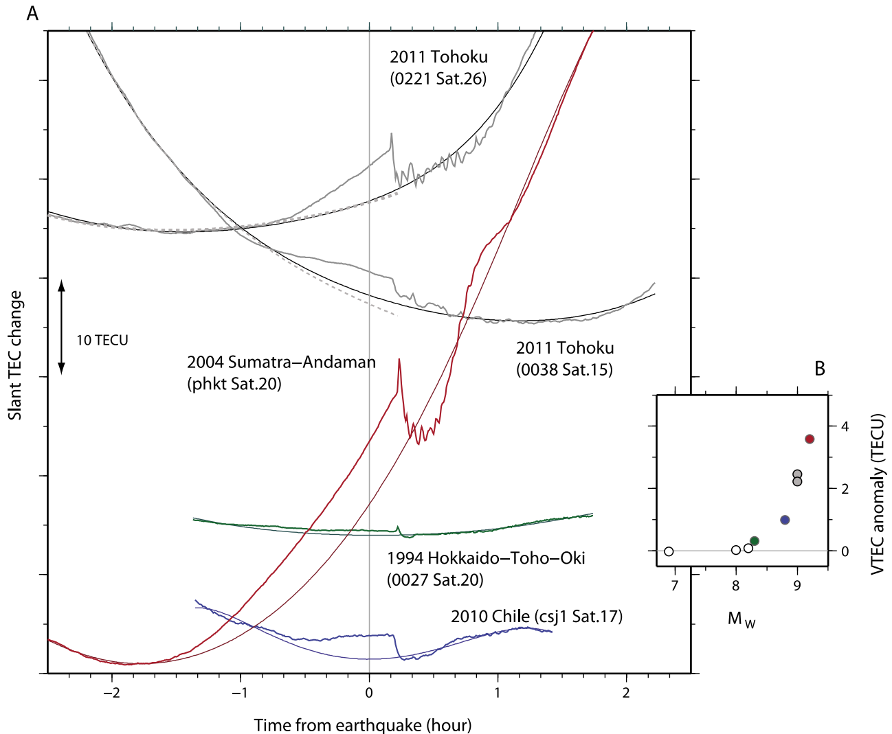
Figure 4. (a) Slant TEC changes and their models in the 2011 Tohoku earthquake, the 2004 Sumatra-Andaman earthquake, the 1994 Hokkaido-Toho-Oki earthquake, and the 2010 Chile (Maule) earthquake. The horizontal axis shows the time from earthquakes. Dashed curves in gray for the top two time series show the models derived with data prior to the possible onset of the precursor (before 5.2 UT) and extrapolated to 5.2–6.0 UT. (b) Vertical TEC anomalies immediately before the earthquakes as a function of their moment magnitudes. Colors correspond to those in Figure 4a. In addition to the five data from four earthquakes in Figure 4a, three smaller earthquakes (Figure S12) are included (white circles).
