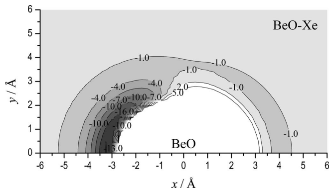
FIG. 1. Two-dimensional contour plot of the potential energy surface (in units of kcal/mol) for BeO-Xe. The internal coordinates of BeO are fixed at the equilibrium values and the origin is set to the center-of-mass of BeO. The positions of Be and O are (-0.85, 0.0) and (0.48, 0.0) , respectively.
