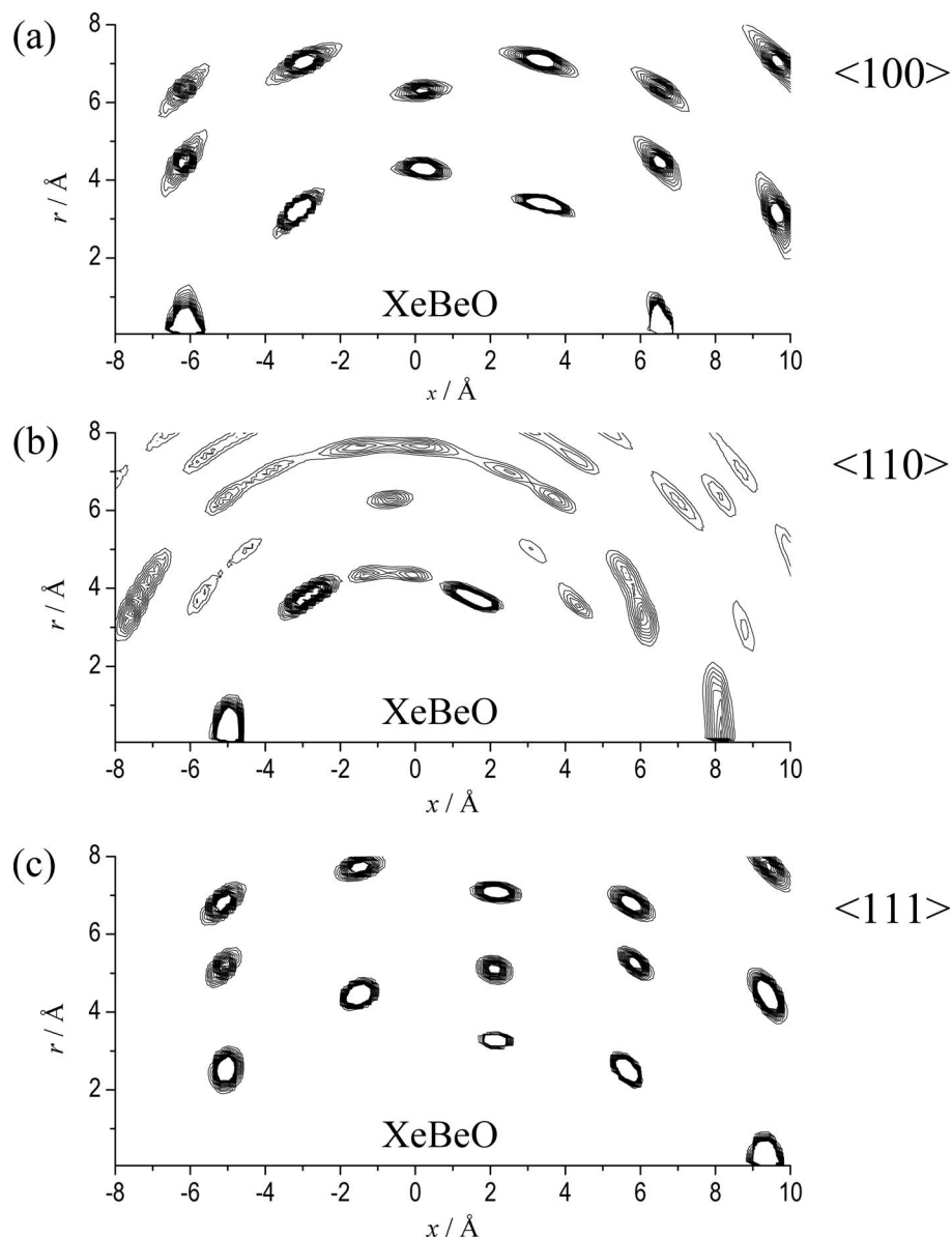
FIG. 5. Contour plots of two-dimensional distribution functions of the Xe atoms around XeBeO for the (a) \langle 100 \rangle , (b) \langle 110 \rangle , and (c) \langle 111 \rangle sites. The positions of XeBeO are the same as those in Figure 3.
