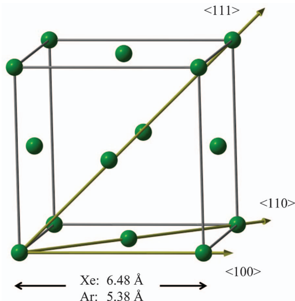
FIG. 4. Fcc lattice structure of solid Xe or Ar. The three possible orientations of RgBeO are depicted as \langle 100 \rangle (four-atomic window), \langle 110 \rangle (nearest neighbor), and \langle 111 \rangle (three-atomic window).
