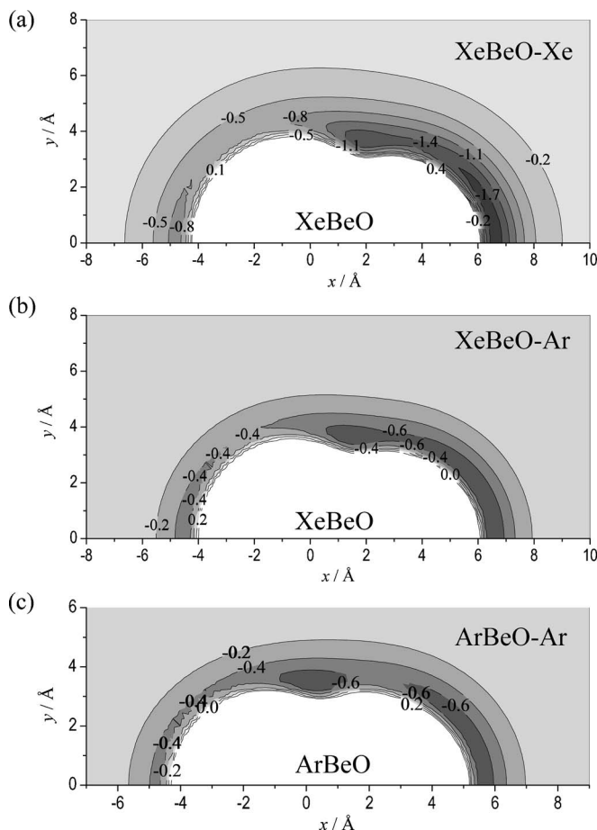
FIG. 3. Two-dimensional contour plots of the potential energy surfaces (in units of kcal/mol) for (a) XeBeO-Xe, (b) XeBeO-Ar, and (c) ArBeO-Ar. The internal coordinates of RgBeO (Rg = Xe or Ar) are fixed at the equilibrium values and the origin is set to the center-of-mass of RgBeO. The positions of the Xe, Be, and O are (-0.51, 0.0) , (1.84, 0.0) , and (3.17, 0.0) , respectively, for XeBeO, and those of the Ar, Be, and O atoms are (-1.12, 0.0) , (0.94, 0.0) , and (2.27, 0.0) , respectively, for ArBeO.
