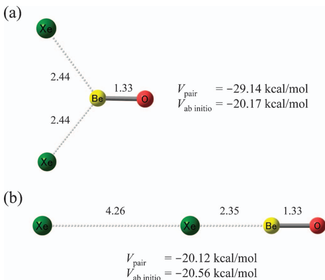
FIG. 2. Minimum energy structures of Xe 2 BeO obtained by (a) the pairwise-additive model and (b) ab initio calculations. Bond lengths are given in unit of Å.
