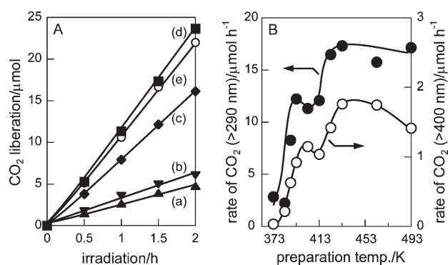
Figure 2. (A) CO 2 liberation for reaction 1 under irradiation at wavelengths >290 nm over (a) BW-373, (b) 383, (c) 388, (d) 393, and (e) 403. (B) Effect of hydrothermal preparation temperature on the CO 2 liberation rate under irradiation at wavelengths (●) >290 nm and (○) >400 nm.
