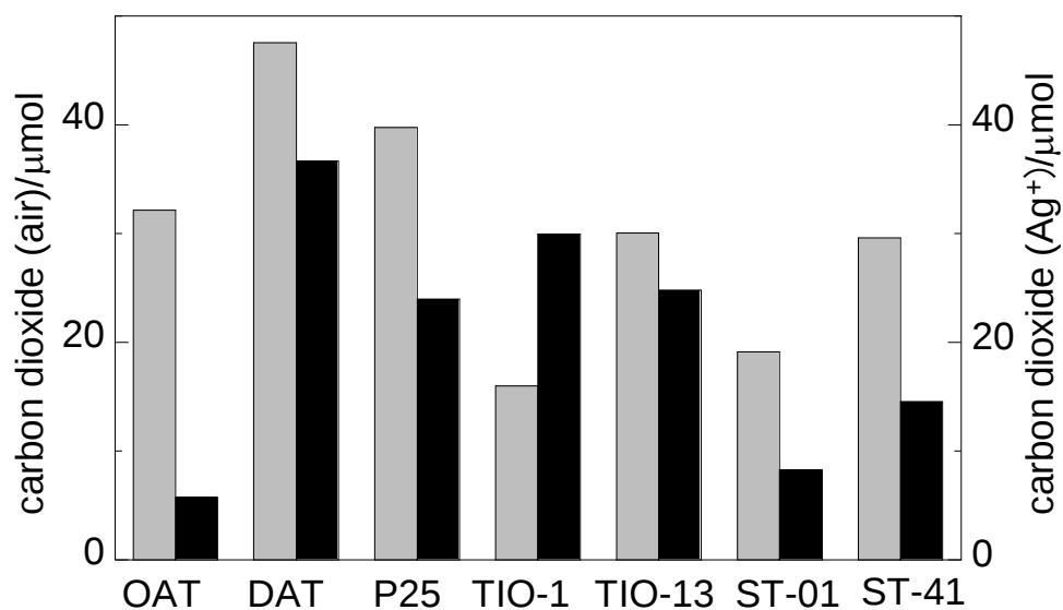
Figure 5 Amount of photocatalytic liberation of carbon dioxide from 5vol% aqueous acetic acid under aerated conditions (left) and under deaerated conditions in the presence of silver ions (250 \mu\text{mol} ) (right) after 1-h photoirradiation. TIO-1, TIO-13, ST-01 and ST-41 are anatase powders with specific surface areas of 73, 65, 327 and 11 \text{m}^2 \text{g}^{-1} , respectively.
