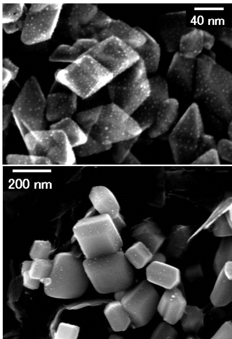
Figure 7 SEM images of silver-photodeposited OAT (upper) and DAT (lower) particles photoirradiated in deaerated aqueous silver sulfate solutions for 80 and 40 min, respectively.
