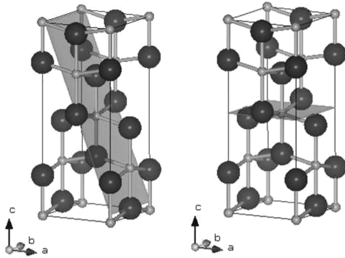
Figure 2 Schematic presentation of (101) (left) and (001) (right) lattice planes in an anatase unit cell. Black and gray balls represent oxygen ( \text{O}^{2-} ) and titanium ( \text{Ti}^{4+} ) ions, respectively.
