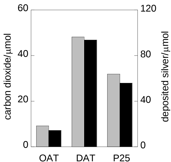
Figure 6 Amount of photocatalytic liberation of carbon dioxide (left) and deposition of silver on the photocatalysts (right) from 5vol% aqueous acetic acid under deaerated conditions in the presence of silver ions ( 250\ \mu\text{mol} ) (right) after 100-h (OAT) and 80-h (DAT and P25) photoirradiation.
