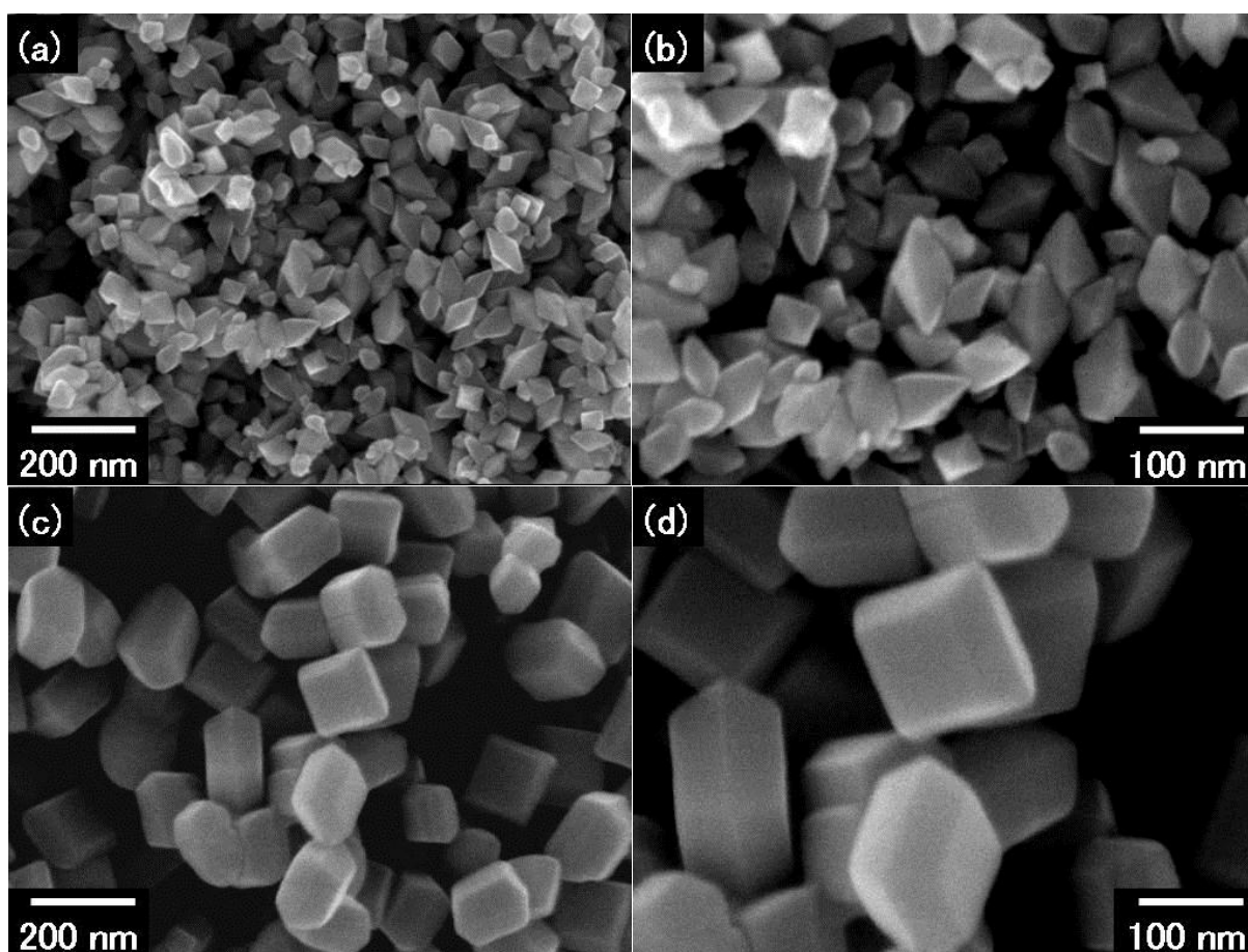
Figure 1 Scanning electron microscopic images of OAT (a, b) and DAT (c, d) anatase single-crystalline particles.
