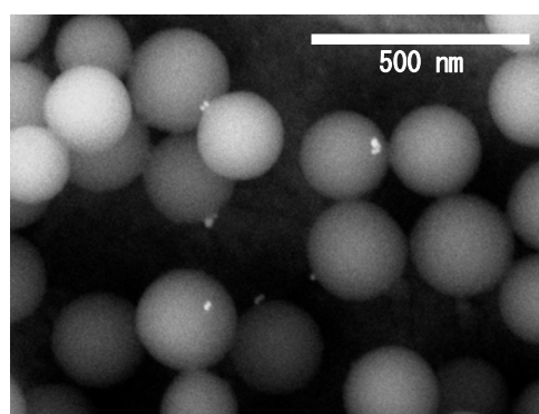
Fig. 3 SEM image of anisotropically gold-nanoparticle-modified silica particles.
