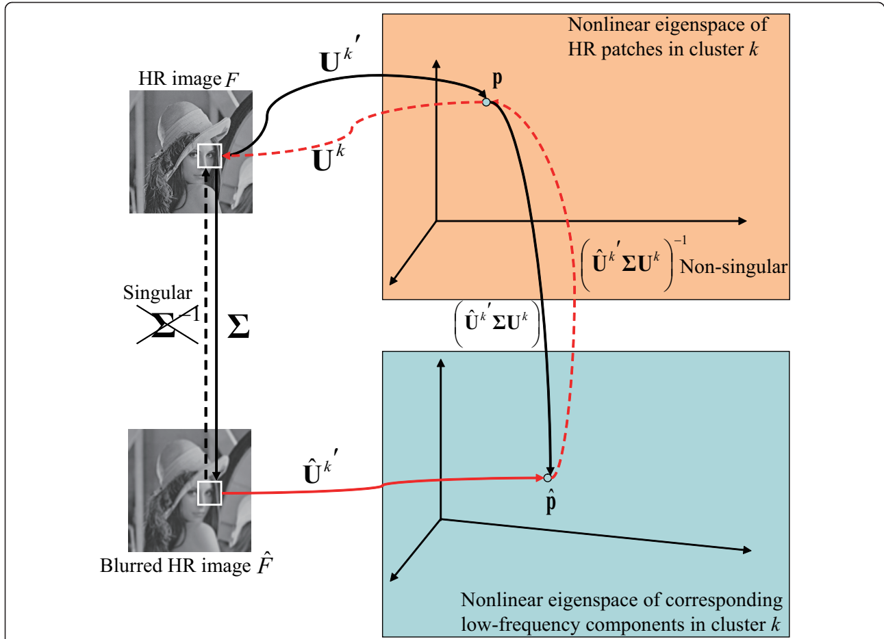
Figure 3 Overview of the algorithm for estimating missing high-frequency components. The direct estimation of HR patches from their LR patches is infeasible since the matrix \Sigma is singular and its inverse matrix cannot be obtained. Thus, the proposed method projects those two patches onto the low-dimensional subspaces and enables the derivation of the projection corresponding to the inverse matrix of \Sigma .
