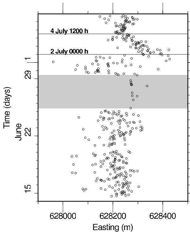
Figure 9. Plot of the evolution of 1 h averaged epicenter easting with time. Shaded zone indicates that only recorder A (easternmost part of the array; see Figure 1) was operating. From 2 July epicenters were located in the easternmost part of the network and then migrated toward the west until 4 July.
