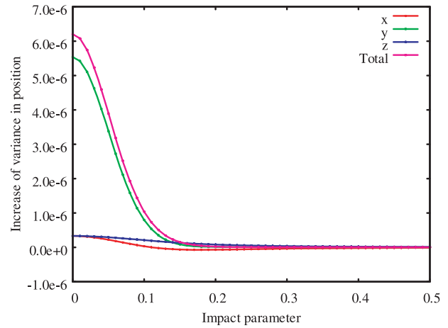
Fig. 3 Incremental variance of a particle in position as a function of classical impact parameter b , in the case of an interaction potential U \propto 1/r due to a point charge at the origin.
