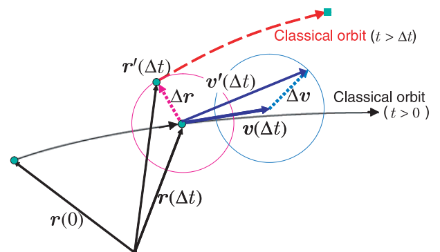
Fig. 1 Semiclassical model for quantum motion. Particle initially at \mathbf{r}(0) classically moves to \mathbf{r}(\Delta t) with a velocity \mathbf{v}(\Delta t) at t = \Delta t - 0 . At this time, it suffers quantum mechanical deviations in position, \Delta \mathbf{r} , and in velocity, \Delta \mathbf{v} . The particle is at \mathbf{r}'(\Delta t) with a velocity \mathbf{v}'(\Delta t) at t = \Delta t + 0 .
