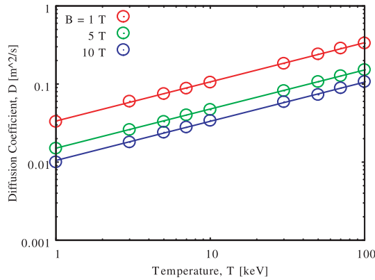
Fig. 5 Case B: Temperature T and magnetic field B dependence of diffusion coefficient D [ \text{m}^2/\text{s} ], with fitting lines in the case of L = \ell_B , the magnetic length.
