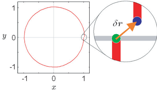
Fig. 2 Deviation of cyclotron motion, \delta \mathbf{r} \equiv \mathbf{r}(\tau_c) - \mathbf{r}(0) , due to uncertainty in one gyration for a given characteristic length L = v_0 \Delta t . Lengths are normalized by the cyclotron radius \rho = mv_0/qB .
