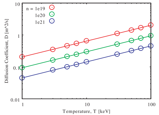
Fig. 4 Case A: Temperature T and density n dependence of diffusion coefficient D [ \text{m}^2/\text{s} ] with fitting lines in the case of L = \Delta \ell , the interparticle separation.
