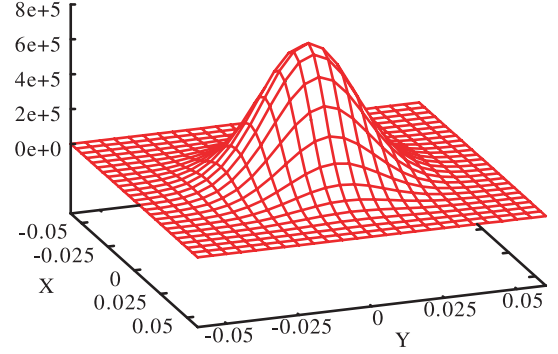
Fig. 3 Histogram for the deviation from the classical position, \delta \mathbf{r} = (\delta x, \delta y) , normalized by the cyclotron radius \rho for N_{MC} = 5 \times 10^7 Monte Carlo trials.
