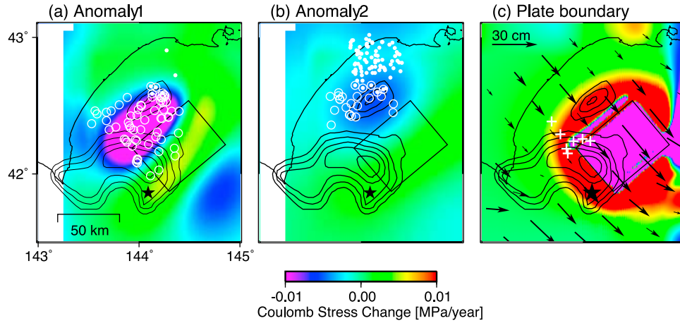
Figure 12. Change in Coulomb failure stress ( \Delta CFS ) in and around the quiescence anomalies. Open and closed white circles indicate the epicenters included in the volume of Anomalies 1 and 2, respectively. (a) \Delta CFS at a depth of 65 km. Epicenters at depths from 50 to 80 km are plotted. The focal mechanism of receiver earthquakes is assumed to be the downdip-extension type: strike = 40^\circ , dip = 80^\circ , and slip = 60^\circ . (b) \Delta CFS at a depth of 100 km. Epicenters at depths from 80 to 110 km are plotted. The focal mechanism of receiver earthquakes is assumed to be the downdip-extension type: strike = 136^\circ , dip = 11^\circ , and slip = -30^\circ . (c) \Delta CFS on the plate boundary. The black star shows a hypocenter of the 2003 Tokachi-oki main shock determined by ISV, and asperities are shown as contours every 1 m of displacement on the fault determined by Yamanaka and Kikuchi [2003]. Arrows indicate the afterslip from 2 October 2003 to 10 November 2003 determined by Ozawa et al. [2004]. Crosses indicate epicenters of the small repeating earthquakes in Region F in Figure 3b of Uchida et al. [2009]. The focal mechanism of receiver earthquakes is assumed to be same as the Tokachi-oki main shock determined by Yamanaka and Kikuchi [2003]: strike = 230^\circ , dip = 20^\circ , and slip = 109^\circ . The rectangle is a projection onto the ground surface of an assumed fault plane of a quasi-static slip with length = 60 km and width = 50 km, which is located on the upper boundary of the Pacific plate. The southwestern point of the fault plane is located at 144.30^\circ\text{E} , 41.87^\circ\text{N} , and depth = 20 km. The fault parameters are assumed to be the same as those for the Tokachi-oki main shock determined by Yamanaka and Kikuchi [2003]: strike = 230^\circ , dip = 20^\circ , and slip = 109^\circ . The displacement is assumed to be 3 cm/year, which is the slip velocity required to build up a seismic moment corresponding to M_w = 6.0 over five years. The displacement of the ground surface caused by a M_w = 6.0 quasi-static slip is too small to detect even if a dense GPS network is deployed on land.
