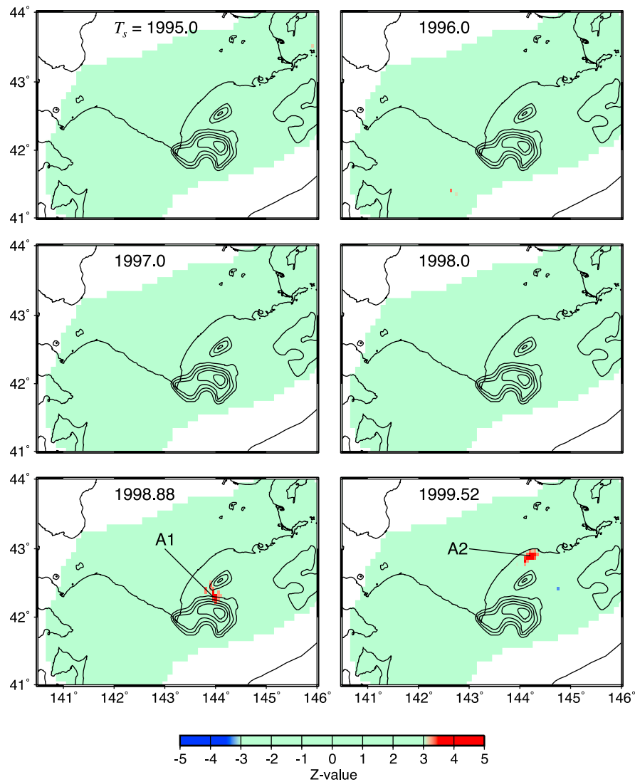
Figure 5. Time slices of Z-value distribution using the re-examined non-declustered catalog. The time window starts at T_s and ends at T_s + T_w , where T_w = 4 years. Only grid points with a radius of the resolution circle smaller than 60 km are selected. The number of such points is 3327. A red color (positive Z-value) and blue color (negative Z-value) represent a decrease and increase in the seismicity rate, respectively. Two alarms with Z-values larger than +3.9 are detected: A1 and A2 (see text). Asperities are shown as contours every 1 m of displacement on the faults for the Tokachi-oki and the Nemuro-oki earthquakes [Yamanaka and Kikuchi, 2003].
