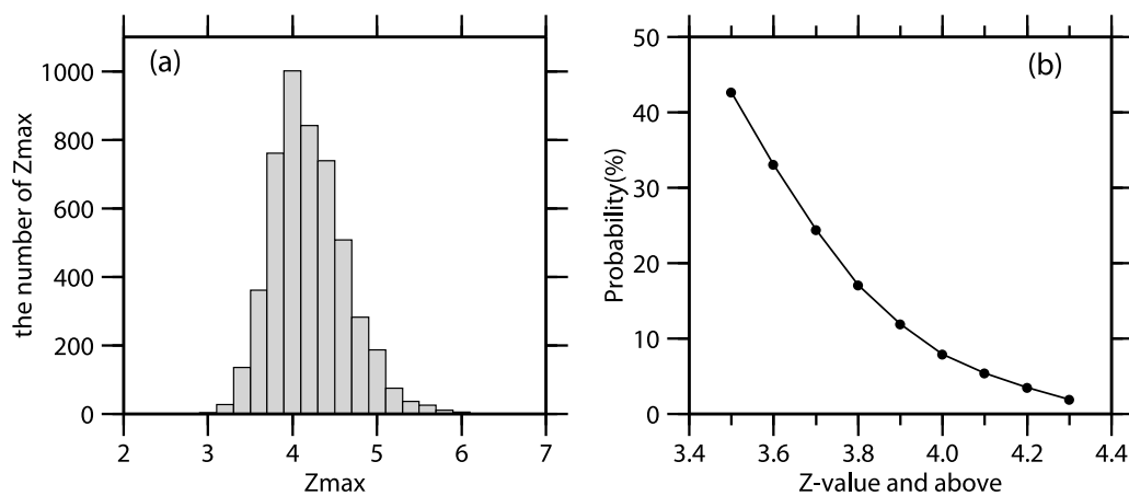
Figure 11. Numerical simulations assuming that earthquakes occur randomly in space and time. 5,000 synthetic earthquake catalogs are produced by UNIX commands. (a) Distribution of Z_{\max} , obtained by the same ZMAP analysis that is applied to the real earthquake catalog. (b) Probability of detection of two spatially separate quiescences with a time difference of less than 0.7 years. The label “Z-value and above” on the horizontal axis means that the two anomalies have Z-values equal to or larger than the values indicated on the axis scale.
