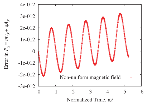
Fig. 1 Numerical Error in momentum in x -direction for non-uniform magnetic field L_B = 5.219 \times 10^{-4} \text{ m} .
