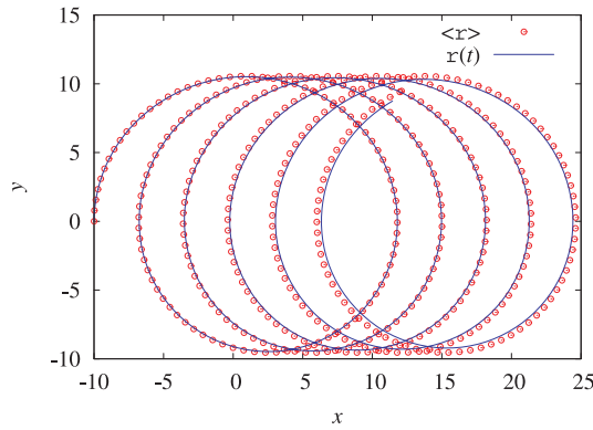
Fig. 3 Comparison of the trajectory of the particle \mathbf{r} in non-uniform magnetic field, L_B = 5.219 \times 10^{-11} m between quantum-mechanical expectation \langle \mathbf{r} \rangle in red, classical orbit \mathbf{r}(t) in blue.
