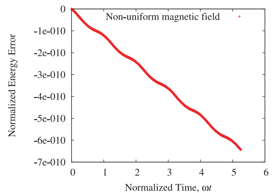
Fig. 2 Numerical error in energy of non-uniform magnetic field with L_B = 5.219 \times 10^{-4} \text{ m} .
