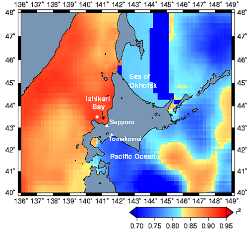
Fig. 4. The spatial distribution of the coefficients of determination between \delta D_{\text{mon}} at Sapporo and the SST mon surrounding Hokkaido. The highest coefficient of determination ( r^2 = 0.92 ) was located in Ishikari Bay (43.5°N, 141°E; denoted by a white diamond), about 40 km from Sapporo (denoted by a white triangle). Lower coefficients of determination (than those in Ishikari Bay) are observed on the Pacific Ocean, close to Tomakomai (denoted by white star) on the southern side of Hokkaido.
