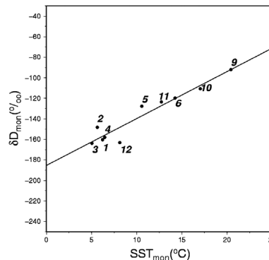
Fig. 5. The correlation between \delta D_{\text{mon}} in Sapporo and SST mon in Ishikari Bay (43.5°N, 141°E).
