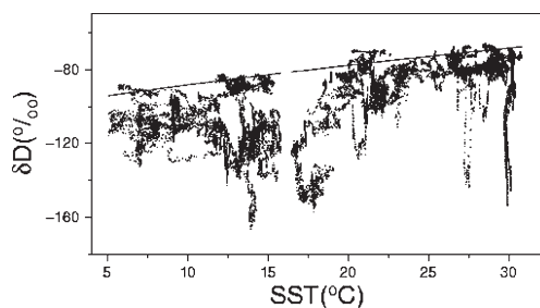
Fig. 6. Relationship between \delta D values near the ocean surface and the SST during the cruise of the T/S Oshoro Maru of the Faculty of Fisheries, Hokkaido University from the Sea of Okhotsk ( 45^{\circ}\text{N} ) to the Pacific Ocean ( 20^{\circ}\text{N} ) from June 8 th to July 15 th 2011. The grey line indicates calculated \delta D of water vapor in equilibrium with ocean liquid.
