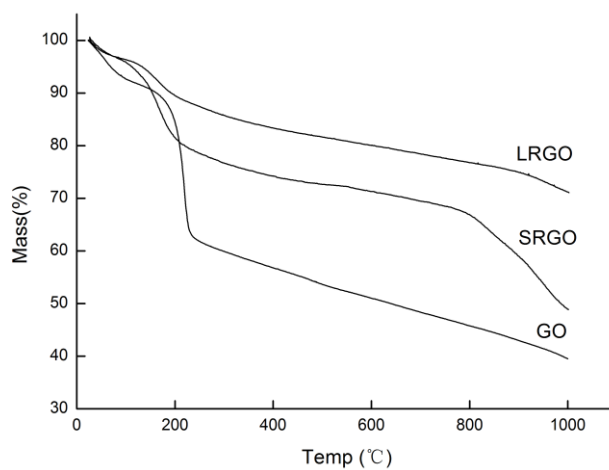
Fig. 14. Thermo-gravimetric analysis for GO, SRGO, and LRGO.
