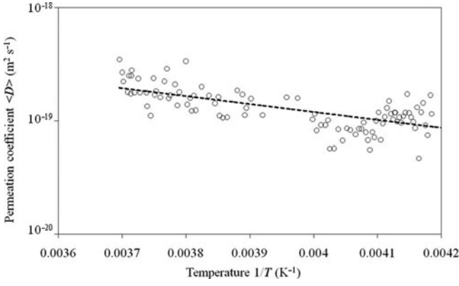
Fig. 7. Temperature dependence of permeation coefficient \langle D \rangle estimated using Equation (1). The dashed line indicates the linear regression implied by Equation (4).
