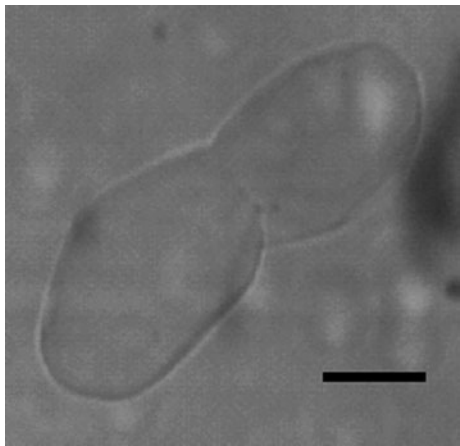
Fig. 5. Irregular type of air-hydrate crystal observed at 2962 m depth, considered to be formed by a two-crystal coalescence (with 100 \mu\text{m} scale bar).
