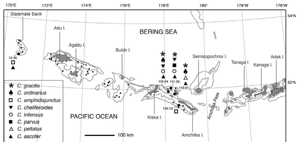
Fig. 1. Map of the western Aleutian Islands (west of Amchitka Pass) and part of the central Aleutian Islands (east of Amchitka Pass). Islands are indicated by dark-gray shading, with the main islands labeled; the 100 m and 500 m depth contours are shown in light gray. Filled circles indicate the 40 sampling stations where bryozoans were collected in 2004, with the smaller filled circles indicating that no specimens of Cauloramphus species were found in the sample. The larger filled circles labeled with station numbers indicate stations where one or more Cauloramphus species were found, with other symbols (key, lower left) indicating the complement of species.
