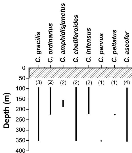
Fig. 9. Summary of known depth ranges of Aleutian Cauloramphus species, inferred from limited sampling data. The number in parentheses above each bar indicates the number of stations at which a species was detected. The hatched area indicates that no sampling was conducted between 0 and 50 m depth.
