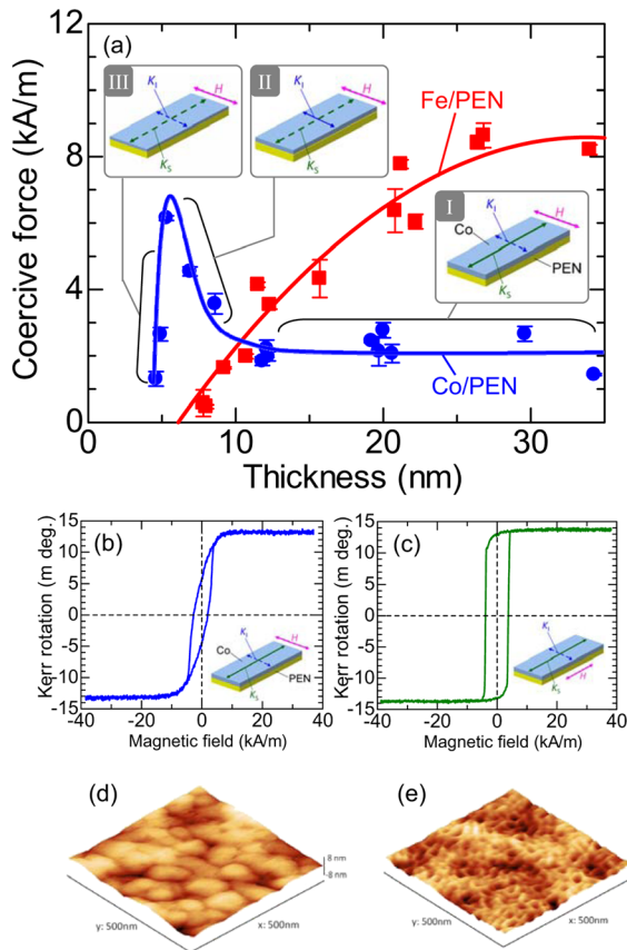
FIG. 3. (Color online) (a) Fe and Co thickness dependences of the coercive force for Fe/PEN and Co/PEN, the magnetization curves with the application of (b) the transverse, and (c) the longitudinal, magnetic field for Co (21 nm)/PEN, and the surface morphologies of (d) Co (6.1 nm)/PEN and (e) Fe (7.8 nm)/PEN.
