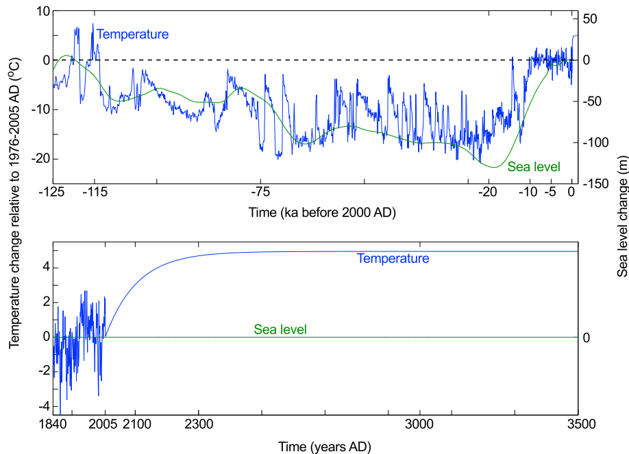
Fig. 2. Surface temperature (blue) and background sea level (green) curves used to drive the ice sheet model simulations. Top panel: full extent of runs (–125 ka to 3500 AD; 2000 AD is indicated by 0); bottom panel: 1840 AD to 3500 AD. Temperature and sea level curves for –125 ka through 1840 AD come from the seaRISE project ( http://websrv.cs.umt.edu/isis/index.php/SeaRISE_Assessment ; seaRISE partners, 2008; Greve et al., 2011) and are based on oxygen isotopes in ocean sediment cores (Imbrie et al., 1984) and in central-Greenland ice cores (Dansgaard et al., 1993; Johnsen et al., 1997). 1840–2005 AD temperatures come from southwestern Greenland observations (Vinther et al., 2006). Future temperatures assume an asymptotic increase to \sim 5 degrees C above 1976–2005 levels, with a time scale of 100 yr (Greve, 2000; see text). Background sea level is held constant from 1840–3500 AD. Labeled tick marks are those referred to in the text and figures; unlabeled tick marks are 25 ka apart in the top panel and 200 yr apart in the lower panel.
