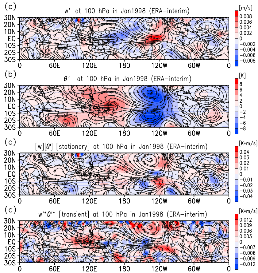
Figure 13. As in Figure 12 but calculated from ERA-Interim.
