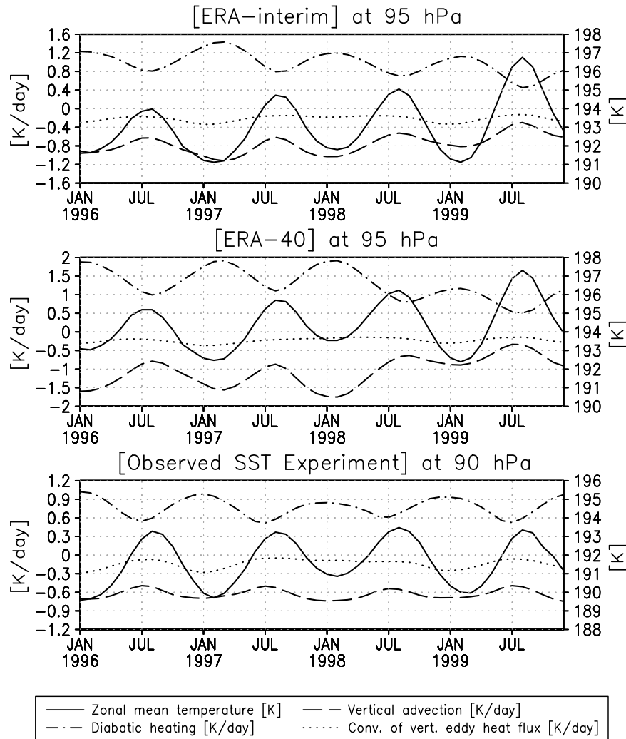
Figure 11. Comparison of the time series of zonal mean temperature (K) and terms in the TEM thermodynamic equation ( \text{K d}^{-1} ) (same plotted terms as in Figures 5 and 6) averaged over the tropics ( 10^{\circ}\text{S} – 10^{\circ}\text{N} ). (top) ERA-Interim at 95 hPa. (middle) ERA-40 at 95 hPa. (bottom) Observed SST experiment at 90 hPa.
