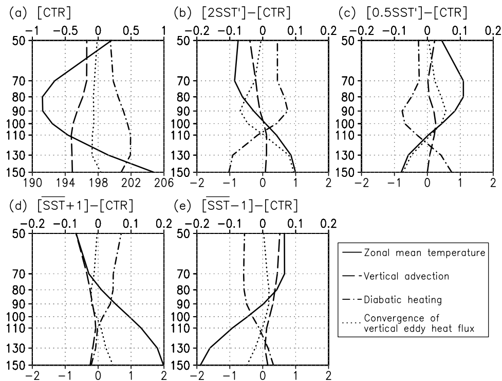
Figure 5. Comparison of annual mean vertical profiles of zonal mean temperature (bottom axis, K) and terms in the TEM thermodynamic equation (top axis, \text{K d}^{-1} ) averaged over the tropics ( 10^{\circ}\text{S} – 10^{\circ}\text{N} ) in (a) CTR and in the difference from CTR of (b) 2\text{SST}' , (c) 0.5\text{SST}' , (d) \overline{\text{SST}} + 1 , and (e) \overline{\text{SST}} - 1 .
