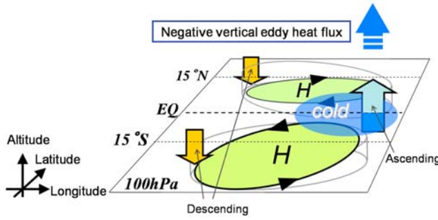
Figure 10. Schematic showing typical wave activity in the tropical western Pacific at 100 hPa. H indicates a high-pressure anomaly, the blue oval is a cold anomaly, the upward arrow is an ascending anomaly, and downward arrows indicate a descending anomaly. These cold and ascending anomalies generate negative vertical eddy heat flux.
