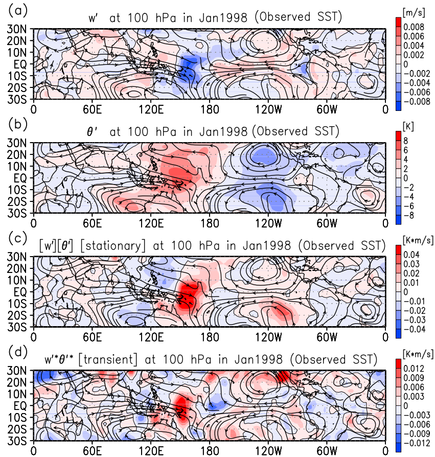
Figure 12. Horizontal field differences in departures from the zonal mean of stream functions (black arrowed contours shown qualitatively): (a) vertical velocity w' , (b) potential temperature \theta' , (c) stationary part of the vertical eddy heat flux [w'][\theta'] , and (d) transient part of the vertical eddy heat flux w'\theta' in the observed SST experiment from climatological means (CTR in January) for January 1998 at 100 hPa.
