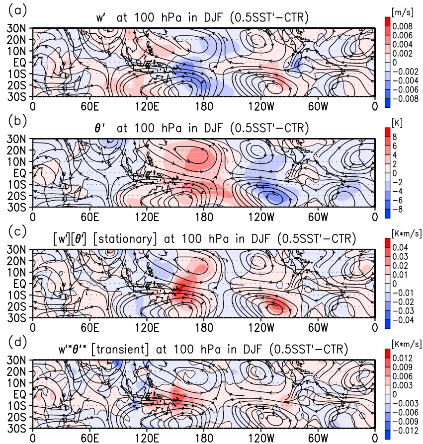
Figure 8. As in Figure 7 but for differences in 0.5SST' from CTR.
