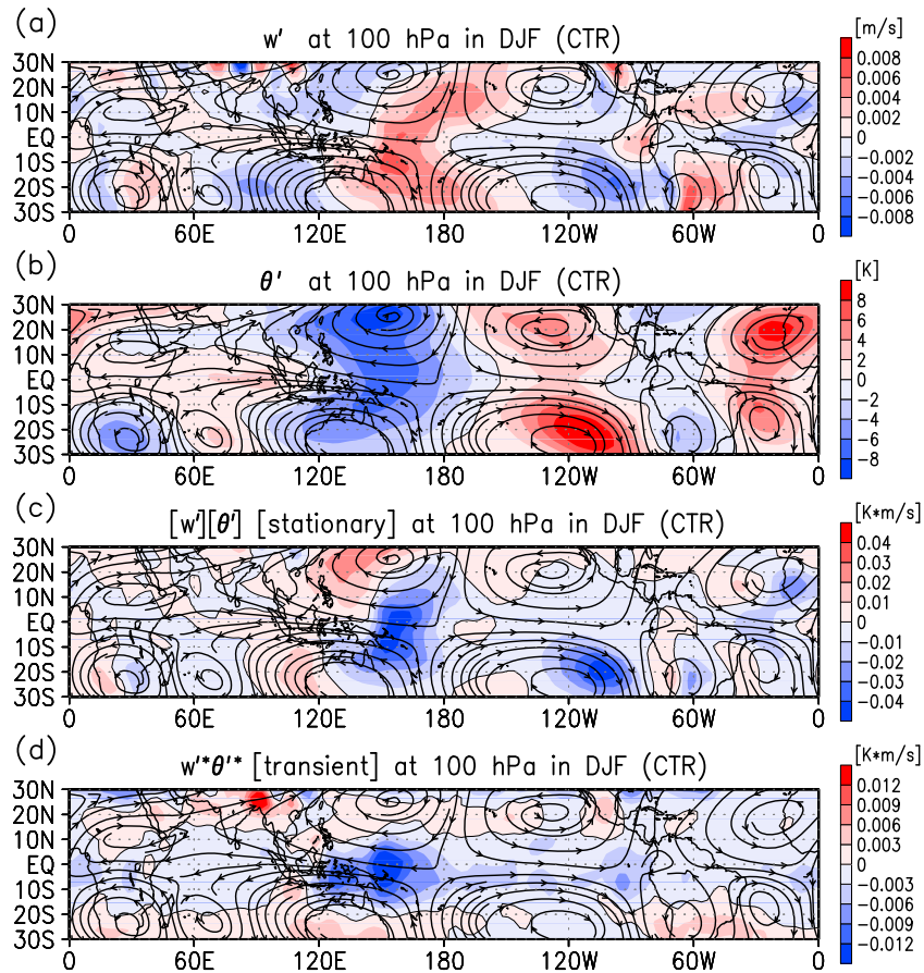
Figure 7. Horizontal fields of departures from the zonal mean of stream functions (black arrowed contours shown qualitatively): (a) vertical velocity w' , (b) potential temperature \theta' , (c) stationary part of the vertical eddy heat flux [w'][\theta'] , and (d) transient part of the vertical eddy heat flux w'^* \theta'^* in CTR for the period December–February at 100 hPa.
