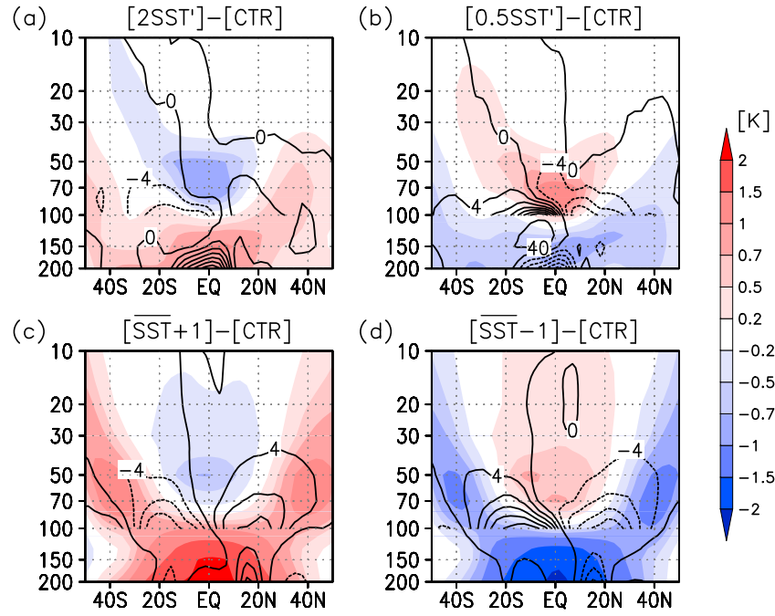
Figure 3. Annual mean cross sections of differences from CTR in zonal mean temperature (K, color bar) and the residual mean stream function ( \text{kg m}^{-1} \text{s}^{-1} , contours) for (a) 2\text{SST}' , (b) 0.5\text{SST}' , (c) \overline{\text{SST}} + 1 , and (d) \overline{\text{SST}} - 1 . The contour interval is 4 \text{ kg m}^{-1} \text{s}^{-1} above 100 hPa and 40 \text{ kg m}^{-1} \text{s}^{-1} below 100 hPa.
