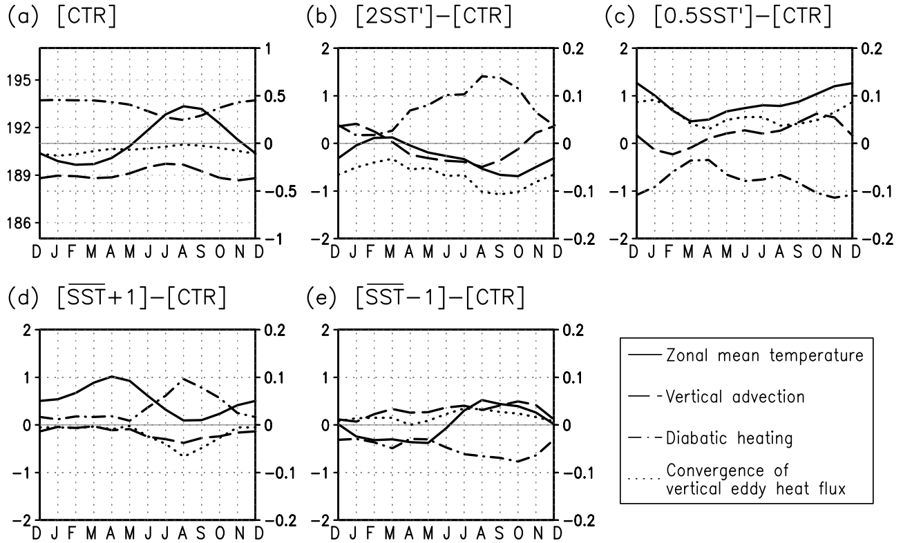
Figure 6. Annual cycles of zonal mean temperature (left axis, K) and terms in the TEM thermodynamic equation (right axis, \text{K d}^{-1} ) (same plotted terms as in Figure 5) in (a) CTR and in the difference from CTR of (b) 2\text{SST}' , (c) 0.5\text{SST}' , (d) \overline{\text{SST}} + 1 , and (e) \overline{\text{SST}} - 1 averaged over the tropics ( 10^\circ\text{S} – 10^\circ\text{N} ) at 90 hPa.
