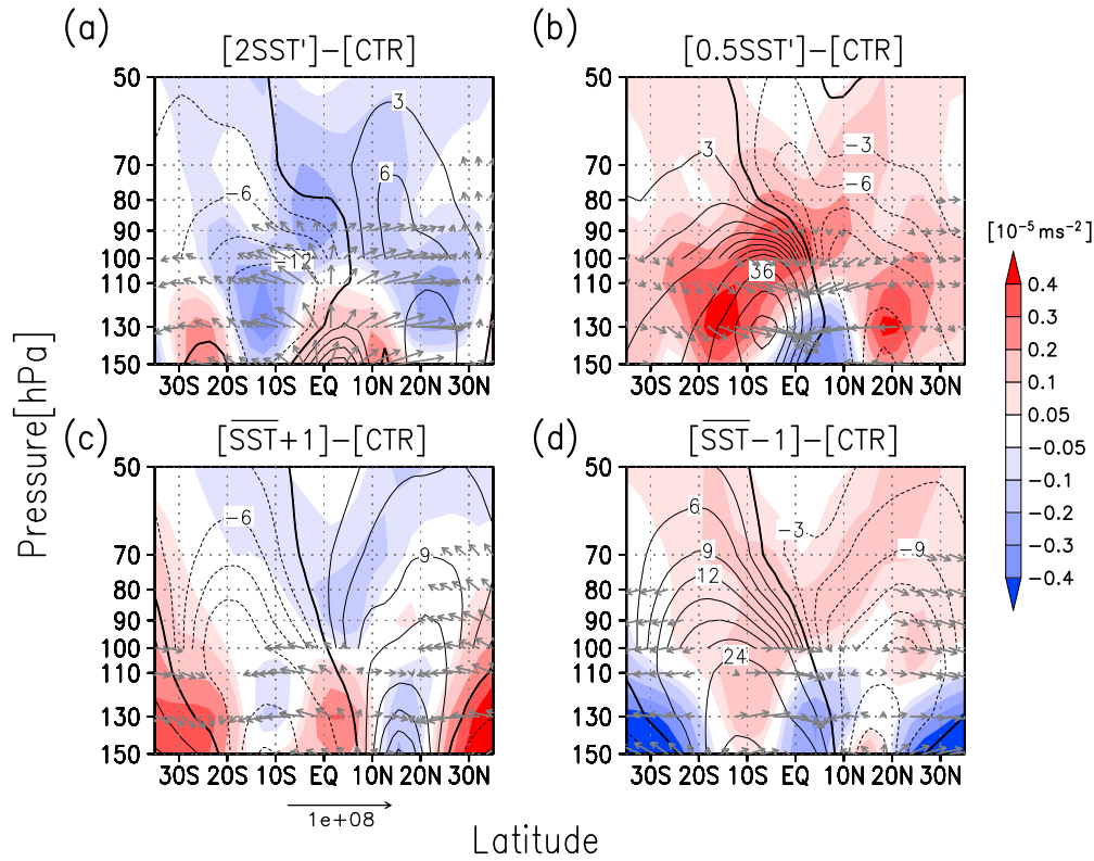
Figure 4. Annual mean cross sections of differences from CTR of the residual mean stream function ( \text{kg m}^{-1} \text{s}^{-1} , contours), the E-P flux ( \text{m}^2 \text{s}^{-2} , arrows), and E-P flux divergence ( \text{m s}^{-2} , color bar) for (a) 2\text{SST}' , (b) 0.5\text{SST}' , (c) \overline{\text{SST}} + 1 , and (d) \overline{\text{SST}} - 1 . The contour interval is 3 \text{ kg m}^{-1} \text{s}^{-1} above 100 hPa and 12 \text{ kg m}^{-1} \text{s}^{-1} below 100 hPa. The vertical component of the E-P flux is multiplied by 200.
