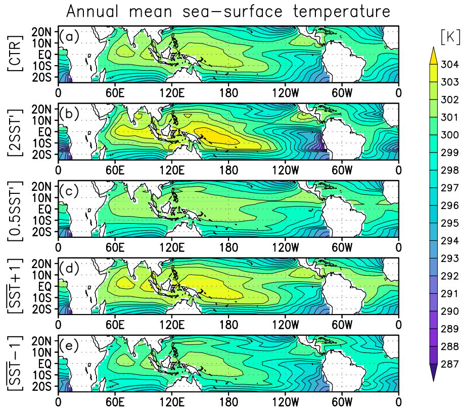
Figure 1. Annual mean sea surface temperature (K) fields used for AGCM experiments. (a) CTR, (b) 2SST', (c) 0.5SST', (d) \overline{\text{SST}} + 1 , and (e) \overline{\text{SST}} - 1 .
