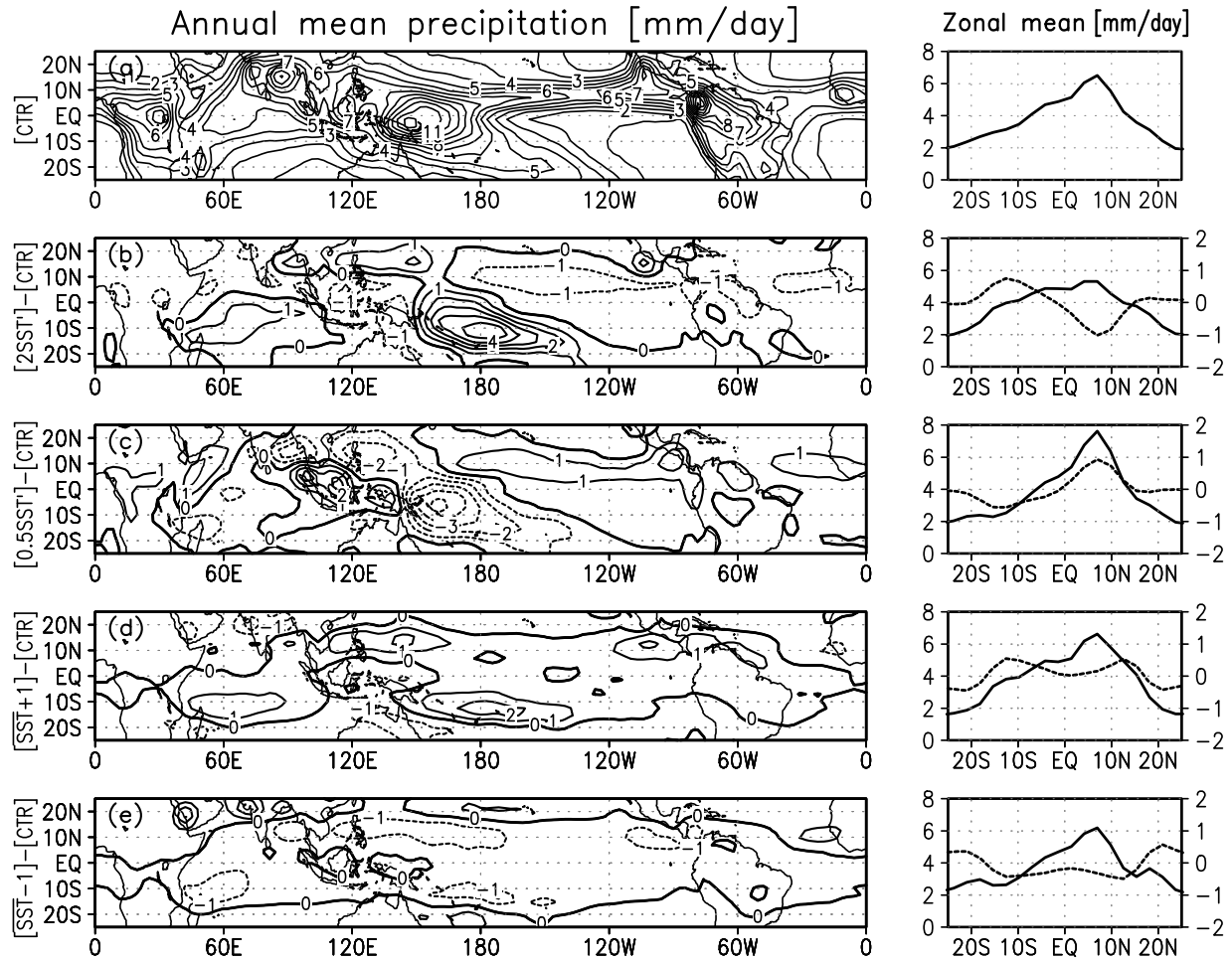
Figure 2. (left) Annual mean precipitation field in (a) CTR and the differences between CTR and (b) 2SST' , (c) 0.5SST' , (d) \overline{SST} + 1 , and (e) \overline{SST} - 1 . (right) Solid lines indicate annual mean zonal mean precipitation in each experiment (left axis), and dashed lines indicate the difference from CTR (right axis).
