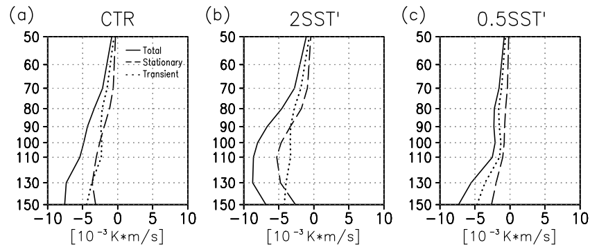
Figure 9. Vertical profiles of annual mean zonal mean vertical eddy heat flux averaged over the tropics (10°S–10°N) between 50 and 150 hPa in (a) CTR, (b) 2SST', and (c) 0.5SST'. Solid lines indicate the total value of the vertical eddy heat flux, dashed lines are the stationary part of the vertical eddy heat flux, and dotted lines are the transient part of the vertical eddy heat flux.
