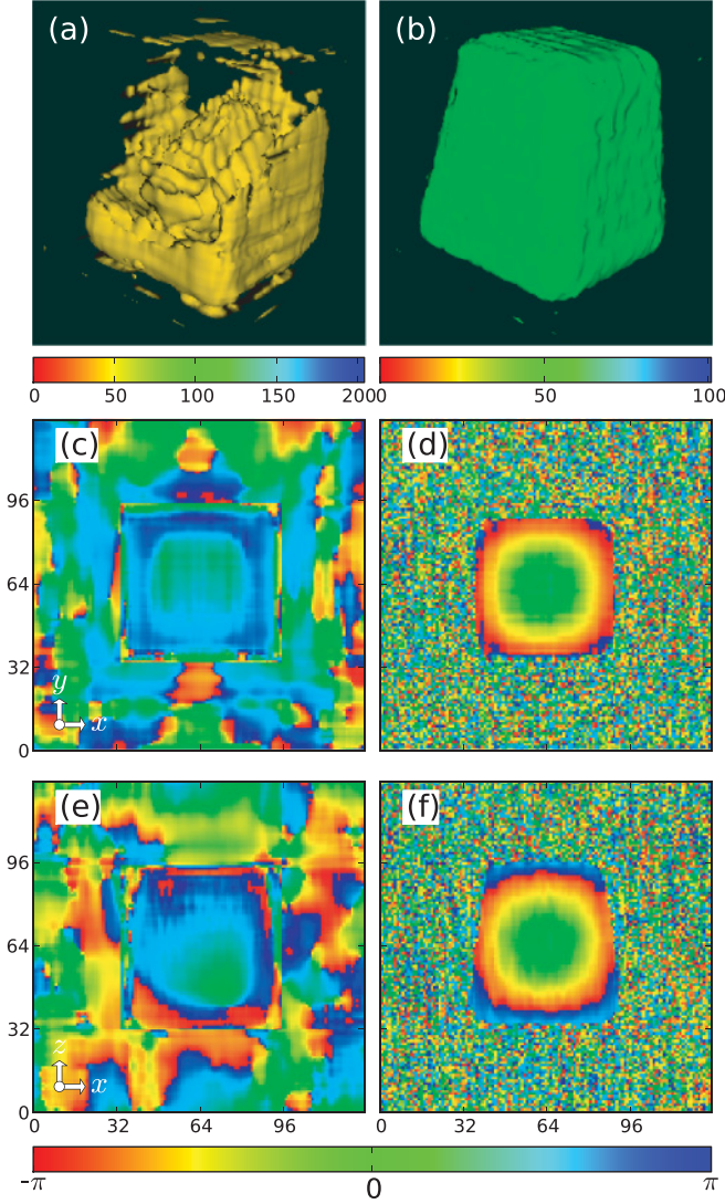
FIG. 3. (Color online) Reconstructed object. Reconstructed amplitude of the object with the (a) HIO and (b) CSHIO algorithms, respectively. Cross sections of the reconstructed phase information for the (c, e) HIO and (d, f) CSHIO algorithms, respectively ( x - y and x - z planes). The HIO algorithm fails to reconstruct the amplitude and phase of the object. The CSHIO algorithm adequately reconstructs both the amplitude and phase of the object. Extraneous phase variations that appear in the HIO phase reconstruction are also suppressed.
