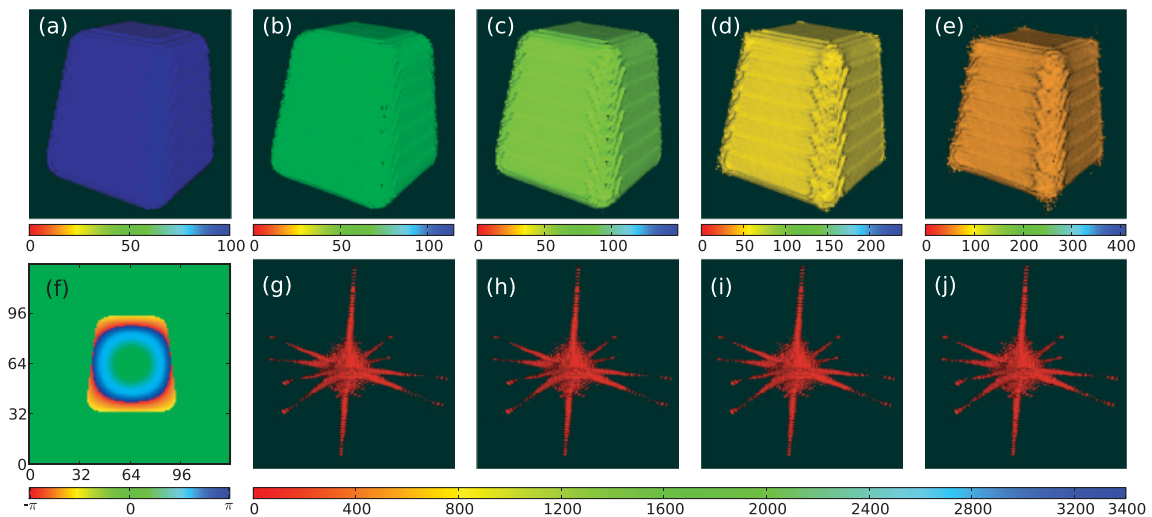
FIG. 2. (Color online) Simulated object with various levels of noise. (a, f) Object in the absence of noise. Phase information is shown as a cross section through the center of the object. (b–e) Object amplitude at an isosurface of 50 with increasing levels of Gaussian noise for which \alpha = 0.1, 0.2, 0.4 , and 0.8 . (g–j) Corresponding Fourier space amplitude of the objects.
