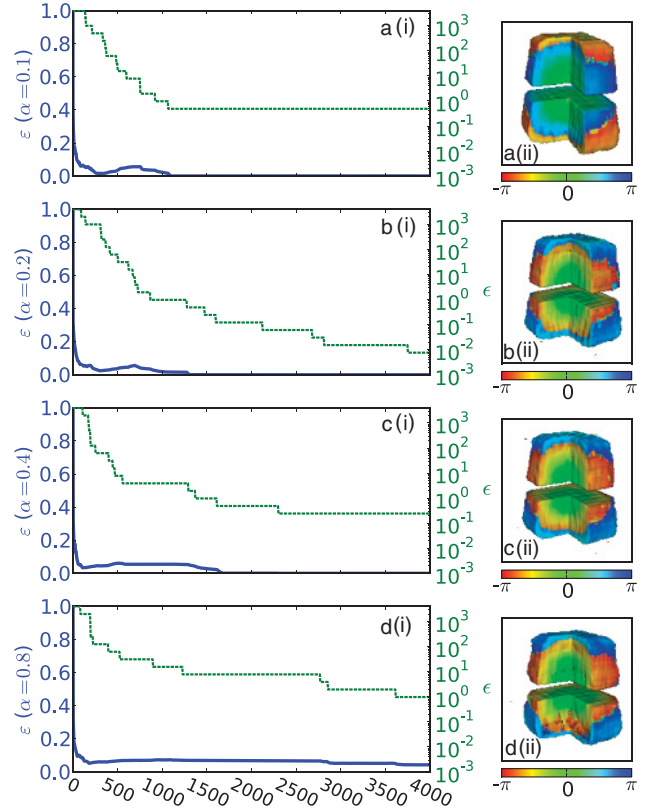
FIG. 4. (Color online) CSHIO reconstructed error. (i) Reconstruction error \epsilon (solid blue line) for the CSHIO algorithm with varying noise levels. The relaxation parameter \epsilon (dashed green line) is also plotted against the right side vertical axis. For noise levels of \alpha = 0.1 to \alpha = 0.4 the error \epsilon is reduced to below 5.0 \times 10^{-4} . (ii) Reconstructed object with the corresponding phase information mapped onto the surface. A quarter section has been removed and the object shown in two halves to aid in visualizing the phase information.
