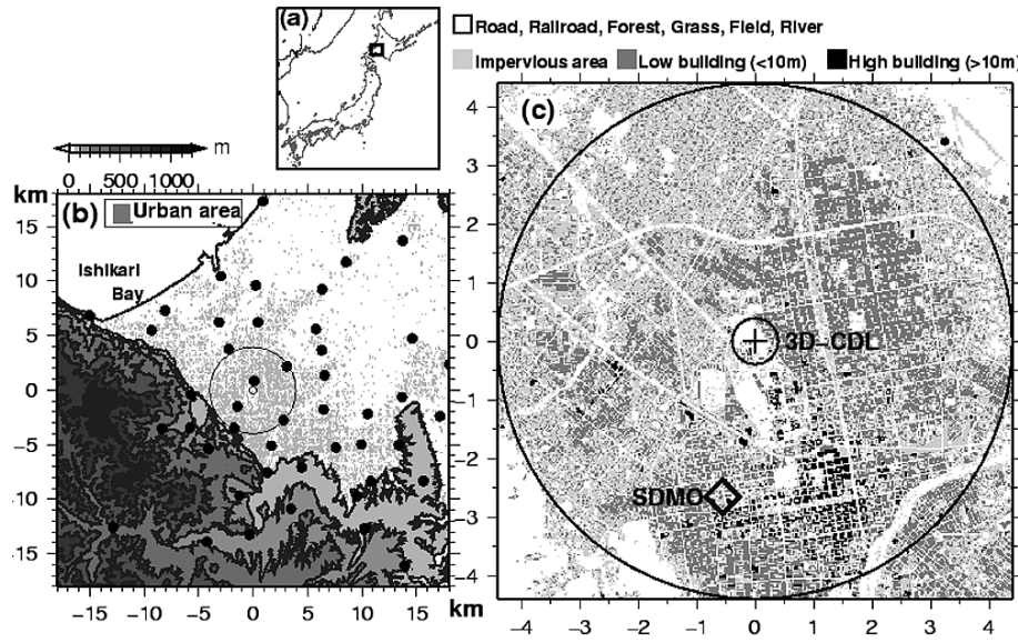
Fig. 1. (a) Location of the 3D-CDL observation area indicated by square. (b) Detailed topographic map of the observational area. Grey contour lines indicate the topography at 0 m, 50 m, 100 m, 200 m, 400 m, 600 m, 800 m, and 1000 m. The 3D-CDL site and its observational area are indicated by small and large circles, respectively. Black dots indicate the location of MULTI stations. (c) Detailed information of land around the 3D-CDL observational area, showing the locations of the 3D-CDL and Sapporo District Meteorological Observatory (SDMO).
