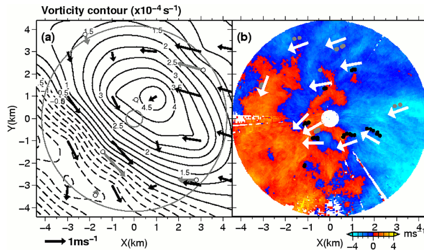
Fig. 4. (a) Wind vector at MULTI stations (grey), interpolated wind vector (black), and distribution of vertical vorticity of the flow (contour; \times 10^{-4} \text{ s}^{-1} ) calculated from interpolated wind vector around the 3D-CDL observation area at 12:30 JST on 4 October 2006. (b) Distribution of averaged Doppler velocity at elevation angle 2.2^\circ in a PPI scan from 12:24 to 12:31 JST and movement of detected dust devil-like vortices. Black and grey dots indicate relatively strong (maximum vorticity more than 0.1 \text{ s}^{-1} ) and weak (maximum vorticity less than 0.1 \text{ s}^{-1} ) vortices, respectively. White arrows indicate movement of vortices.
