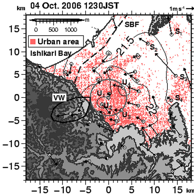
Fig. 3. Horizontal distribution of air temperature (contour line) and wind vector of MULTI at 12:30 JST on 4 October 2006. A grey circle indicates the observational area of the 3D-CDL. The dashed line and solid closed curve indicate the sea-breeze front (SBF) and the valley wind (VW), respectively.
