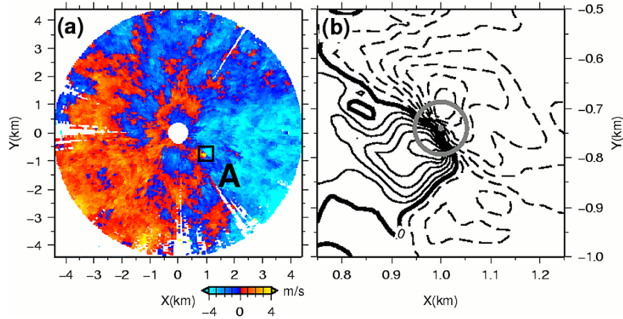
Fig. 2. (a) Doppler velocity at elevation angle 2.2^\circ in PPI scan and detected Vortex A at 12:26 JST on 4 October 2006. (b) Close-up view of the Doppler velocity for Vortex A. The contour interval is 1 \text{ m s}^{-1} . Thick solid lines indicate a zero value, and thin solid (dotted) lines show positive (negative) values. The deduced core diameter of the vortex is shown by a grey circle.
