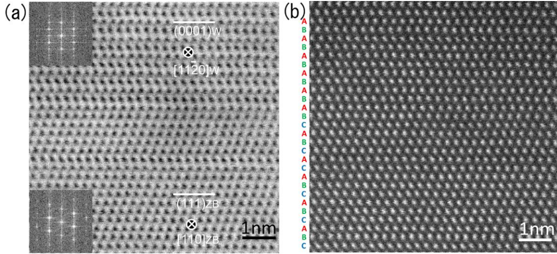
Figure 3 (a) BF-STEM image of GaON nanowire. Incident electron beam along [11-20] and [110] zone axes in hexagonal wurtzite and its corresponding cubic zinc-blende lattice. (b) HAADF-STEM image of GaON nanowire. A, B and C indicate the stacking sequences.
