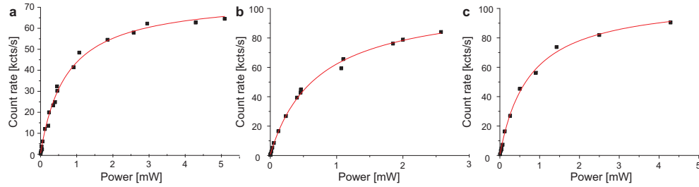
Fig. 4. (a,b,c) Saturation measurements of the NV from Fig. 2(c). Fitting (red solid lines) was done according to text. This analysis reveals (a) 74 \pm 2 kc/s, (b) 104 \pm 1 kc/s and (c) 107 \pm 3 kc/s for collection via the objective, fiber end one and fiber end two, respectively (see Fig. 1(a)). In total 211 \pm 3 kc/s single-mode single photons from the fiber were measured. The efficiencies to measure a single photon from the tapered region are \nu = 0.33 for emission from fiber end one and \nu = 0.29 for fiber end two. Taking these efficiencies into consideration, a total number of (689 \pm 12) \cdot 10^3 single photons are coupled to the single-mode fiber at saturation intensities.
