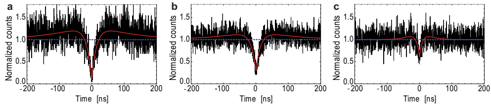
Fig. 3. (a) Normalized auto-correlation function of the same single NV center as in Fig. 2(c). Light was collected via the air objective (see Fig. 1(a)). A deep anti-bunching dip g^{(2)}(0) = 0.11 is visible. According to the spectrum in Fig. 2(c) this correlation measurement confirms a single neutral NV defect center as single photon source. (b) Cross-correlation measurement for fiber end one with the photons collected via the objective (see Fig. 1(a)). g^{(2)}(0) = 0.29 proves single photon statistics for the fiber coupled light. For an equivalent measurement for fiber end two g^{(2)}(0) was 0.29 (not displayed for redundancy). (c) Cross-correlation measurements between the two fiber ends. The anti-bunching dip g^{(2)}(0) = 0.61 is slightly higher than 0.5, yet indicating strong quantum character of the light. The correlation functions in (a), (b), (c) were taken at excitation intensities of 450 \mu\text{W} , 500 \mu\text{W} and 400 \mu\text{W} , respectively.
