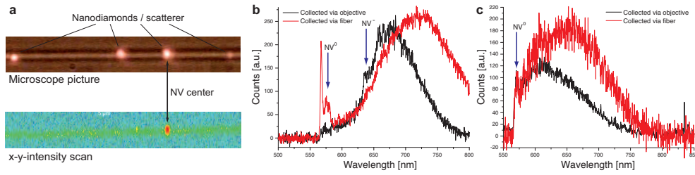
Fig. 2. (a) Top: Microscope picture of a 40 \mu\text{m} long tapered fiber section. Laser is guided through the fiber. The scattered light from four scatterers is visible. Bottom: x-y-intensity scan of the same region. While the tapered fiber is scanned, 532 nm laser light is focused on the tapered fiber. The laser is blocked with a 565 nm long pass filter before the detection of fluorescence > 565 nm. One of the four scatterers contains several nitrogen vacancy centers. (b) Spectrum of the fluorescence of the light emitter depicted in the lower panel of Fig. 2(a) at excitation intensity of 500 \mu\text{W} . Several nitrogen vacancy centers contribute to the emission. Clearly visible are the zero phonon lines of the neutral (575 nm) and the negatively charged (637 nm) centers. (c) Spectrum of the fluorescence of a single neutral nitrogen vacancy center excited with 500 \mu\text{W} , normalized to the zero phonon line at 575 nm. The black and red line in (b) and (c) represent the fluorescence collected via an air objective and via one end of the fiber, respectively. The red spectra appear redshifted due to chromatic dependence of the fiber filter stage transmission.
