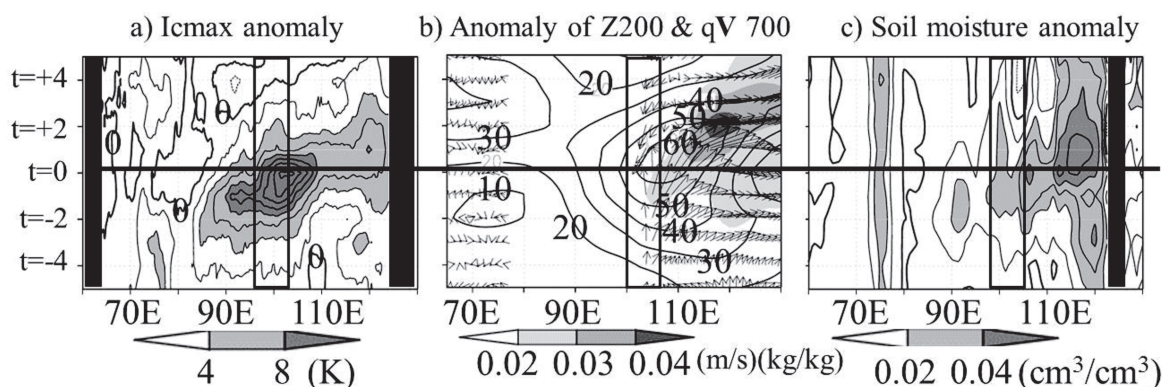
Fig. 9. Time evolution (from t = -5 to t = +5 ) of composite anomaly averaged between 30^{\circ}\text{--}35^{\circ}\text{N} of a) I_{\text{cmax}} (contour interval is 2 K), b) geopotential height at 200 hPa (gpm, contour), qV at 700 hPa ( \text{m s}^{-1} \times \text{kg kg}^{-1} ; vector), and magnitude of qV ( \text{m s}^{-1} \times \text{kg kg}^{-1} ; shaded), and c) soil moisture (contour interval is 0.01 \text{ cm}^3 \text{ cm}^{-3} ) for the LMCS case of Area 2. A horizontal thick line means t = 0 , and an open square indicates the longitude of Area 2. The black shaded area in Figure a and c is an area from which no data was obtained.
