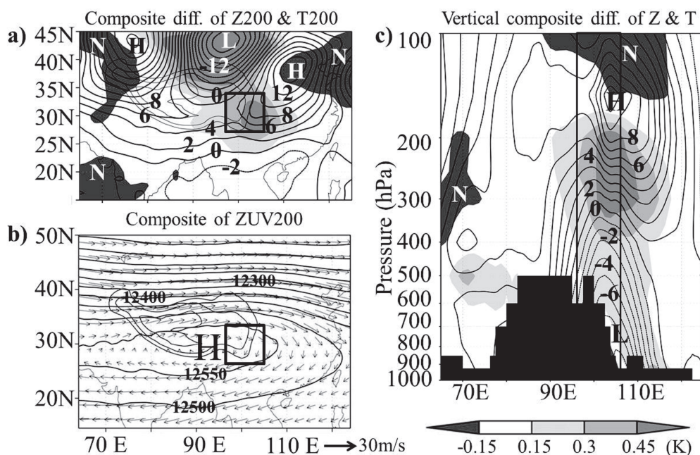
Fig. 3. a) Composite diff. of the temperature (shaded, K) and geopotential height (contour, gpm) at 200 hPa, b) composite distribution of the wind (vector, \text{m s}^{-1} ) and geopotential height (contour, gpm) at 200 hPa, and c) longitude-vertical cross section of the composite diff. of temperature (shaded, K) and geopotential height (contour, gpm) along 30°N in the LMCS cases of Area 2. The scale of shades in Fig. 3a is the same as that in Fig. 3c. “L,” “H,” and “N” indicate “a low geopotential height anomaly,” “a high geopotential height or its anomaly,” and “a negative value of temperature anomaly,” respectively. The topography is masked out with black in Fig. 3c.
