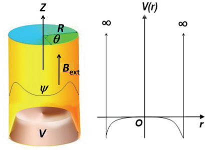
FIG. 1 Schematic picture of cylindrical nanowire system and a cross-sectional potential diagram, where O indicates the reference of the energy.
