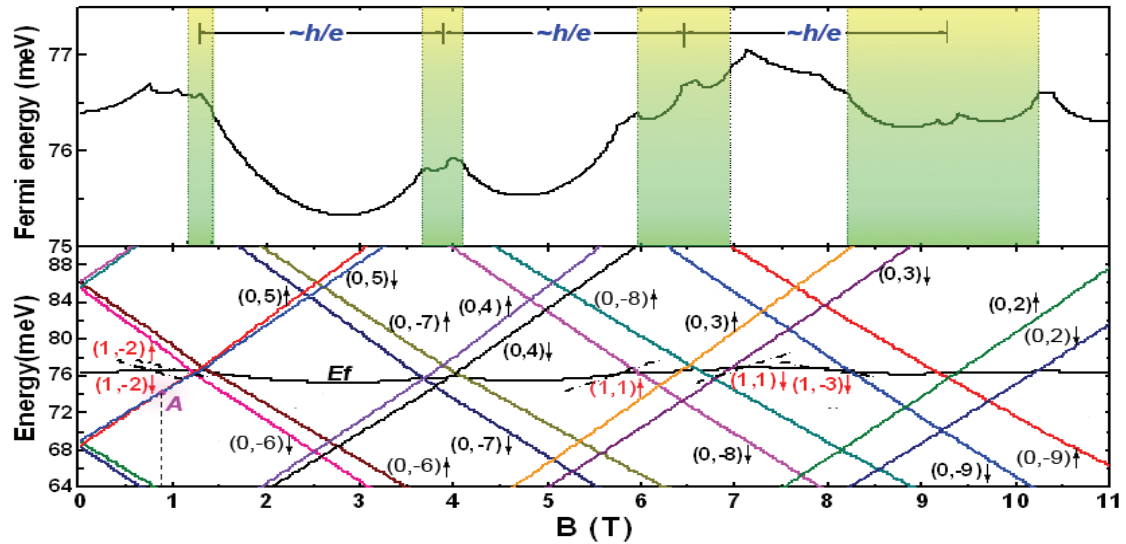
FIG. 2 Lower panel: The calculated first subband energy levels ( m=0 ) for an InAs nanowire (60 nm in diameter) as a function of magnetic field along the wire. The crossing points by various angular momentum states with subband index due to the radial confinement m=1 are indicated by black dash lines. Upper panel: Zoom-in section of the Fermi energy as a function of B . The clusters of the crossings with m=0 distribute in the yellow-green shaded regions. The distance between the middle lines of two yellow-green regions is h/e in magnetic flux.
