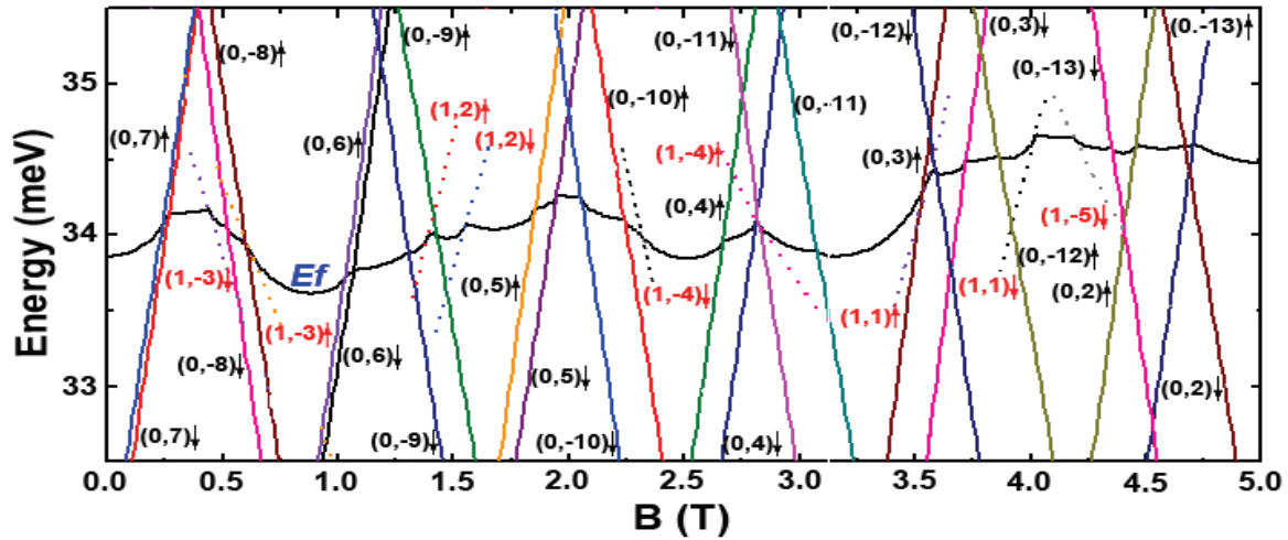
FIG.3 Energy level structure near Fermi energy for 100 nm wire with 3D N_{3D}=2 \times 10^{23} \text{ m}^{-3} .
