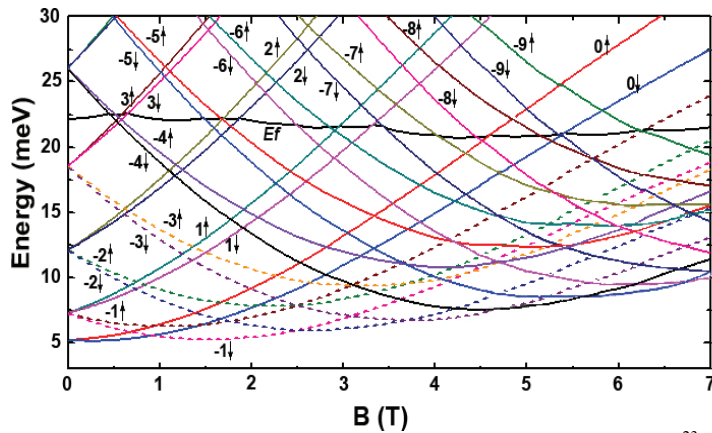
FIG.4 All the subband structure in 100 nm wire with 3D N_{3D}=0.5 \times 10^{23} \text{ m}^{-2} .
