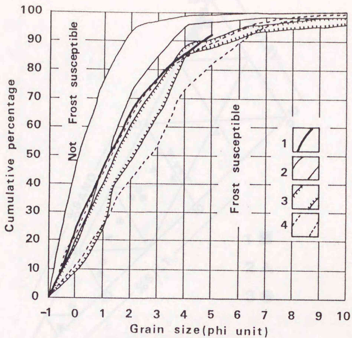
Figure 24 Grain size distribution of matrix of slope deposits in the study area. 1: limit of frost susceptibility (Beskow, 1935), 2: matrix of slope deposits in the granite area, 3: matrix of slope deposits in the hornfels area, 4: matrix of slope deposits in the shale area.
