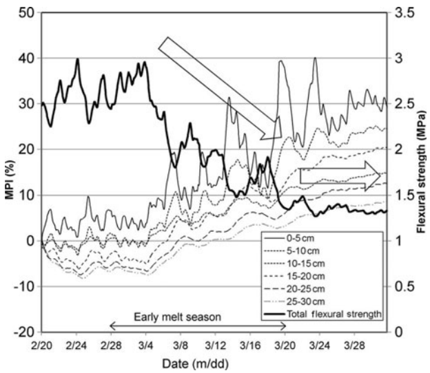
Fig. 16. Time series of MPI at each level and the total ice flexural strength, estimated from numerical modeling. Dates are month/day in 2009.
