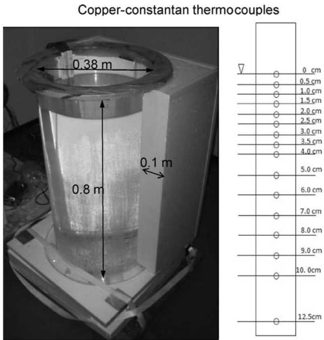
Fig. 7. Apparatus of the tank experiment. The tank was covered with 0.1 m thick Styrofoam to avoid freezing at the side wall and bottom. The copper–constantan thermocouples were mounted on the side wall to monitor the temperature profile. The right-hand panel shows the measurement depths.
