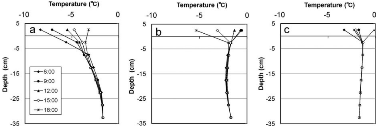
Fig. 13. Evolution of computed temperature profiles on (a) 20 February 2009, (b) 7 March 2009 and (c) 24 March 2009.
