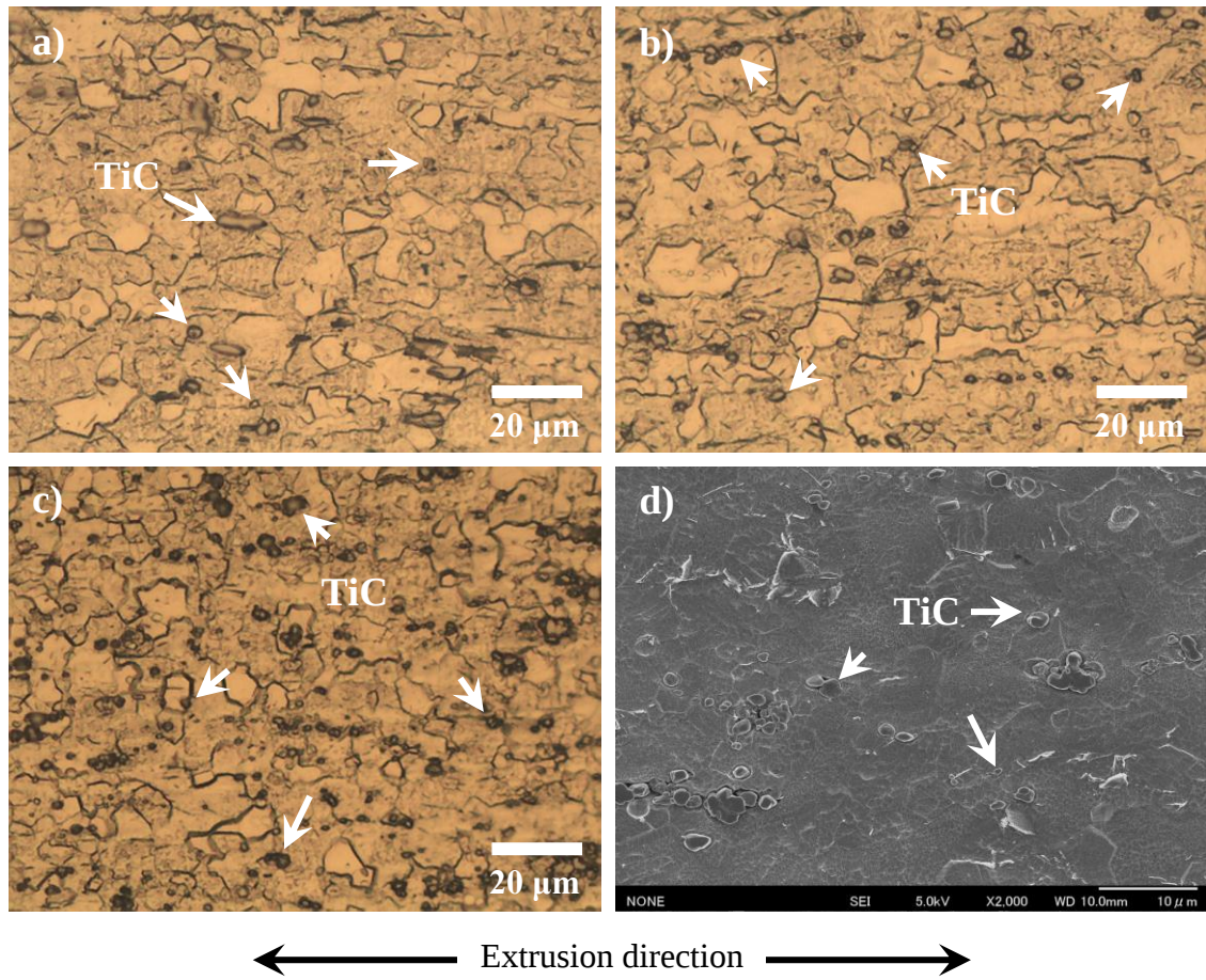
Fig. 6 Optical microstructures of the extruded pure Ti coated with (a) 1.0, (b) 2.0 and (c) 3.0 wt.% CNT/zwiterionic solutions after annealing at 473 K for 360 ks and (d) SEM microstructure at necking area of sample (c) after tensile testing at 673 K
