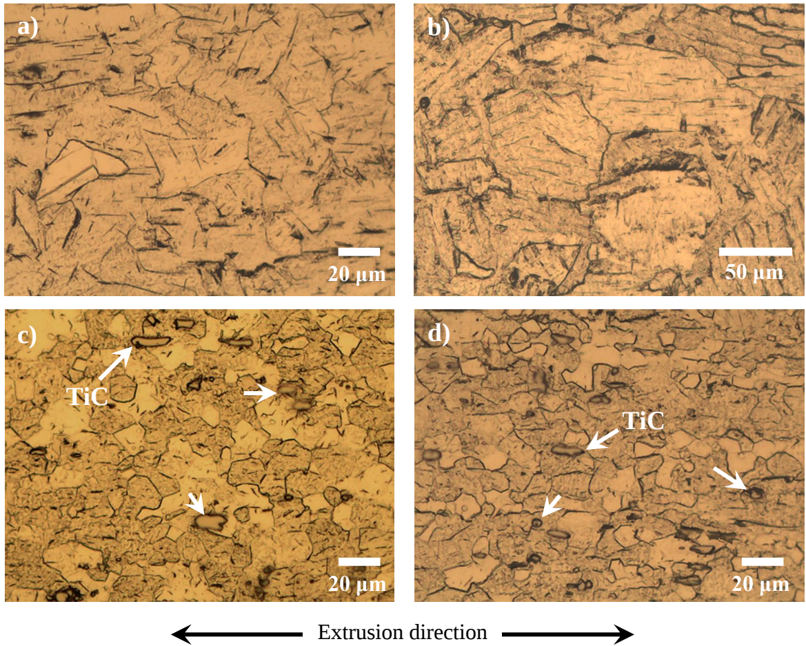
Fig. 2 Optical microstructures of the extruded pure Ti material without CNTs reinforcement (a) before and (b) after annealing at 473 K for 360 ks, compared to microstructure of the extruded pure Ti/CNT composite coated by 1.0wt.%CNTs/zwitterionic solution (c) before and (d) after annealing at 473 K for 360 ks.
