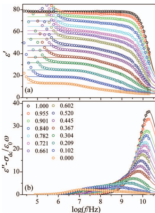
FIG. 2. Frequency dependence of (a) dielectric constant and (b) dielectric loss after subtraction of dc conductivity of water, TX-100/bmimPF 6 mixture, and ILMs with different water content. The solid lines are best fits.
