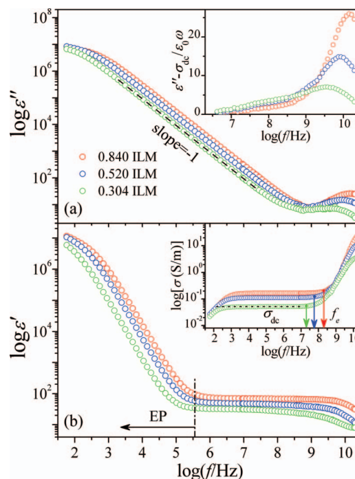
FIG. 1. Frequency dependence of (a) dielectric loss and (b) dielectric constant of 0.840, 0.520, and 0.304 ILMs in the frequency range from 40 Hz to 20 GHz. The insets in (a) shows the frequency dependence of the dielectric loss after subtracting the dc conductivity. The inset in (b) shows the frequency dependence of conductivity, where the arrows indicate the hopping frequency, see text.
