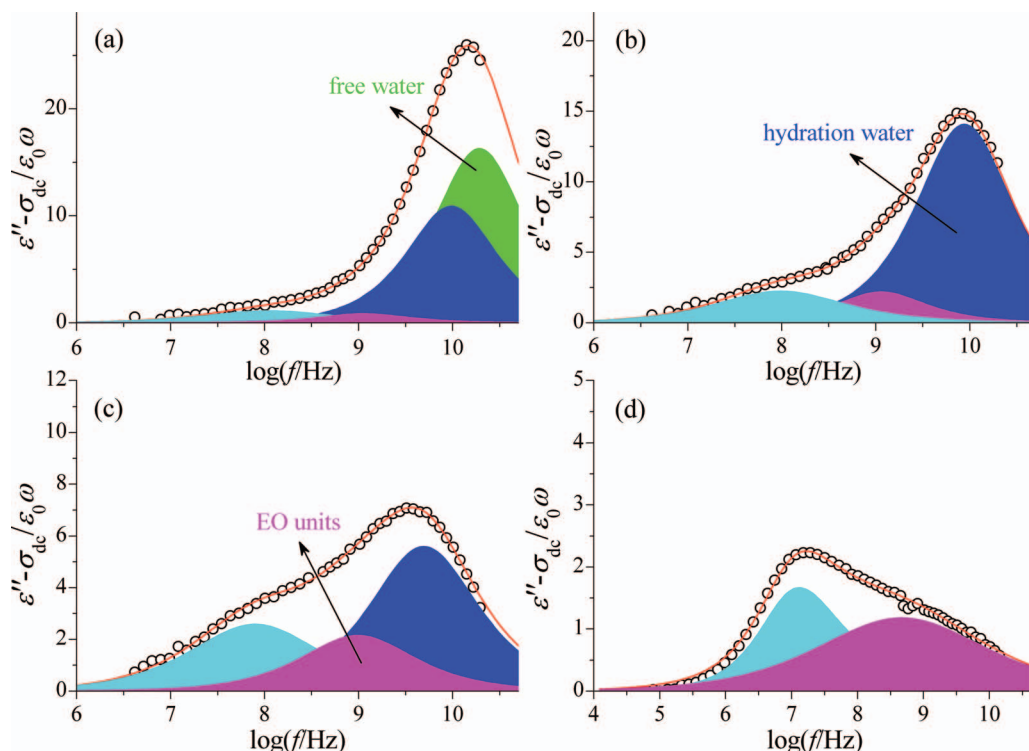
FIG. 4. Fitting results of the dielectric loss curves of (a) 0.840 ILM, (b) 0.520 ILM, (c) 0.304 ILM, and (d) TX-100/bmimPF 6 mixture. The solid lines are the total fitting results and the filled area with different color represents the contribution of different relaxation.
