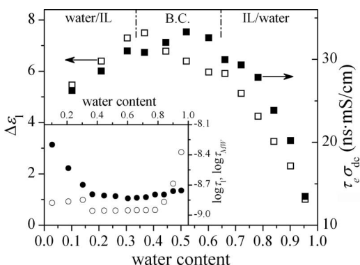
FIG. 8. Water content dependence of the dielectric increment of the low frequency relaxation (open squares) and the product of the hopping time and dc conductivity (filled squares). The inset shows the water content dependence of the relaxation time of the low frequency relaxation (filled circles) and the calculated Maxwell-Wagner relaxation time (open circles).
