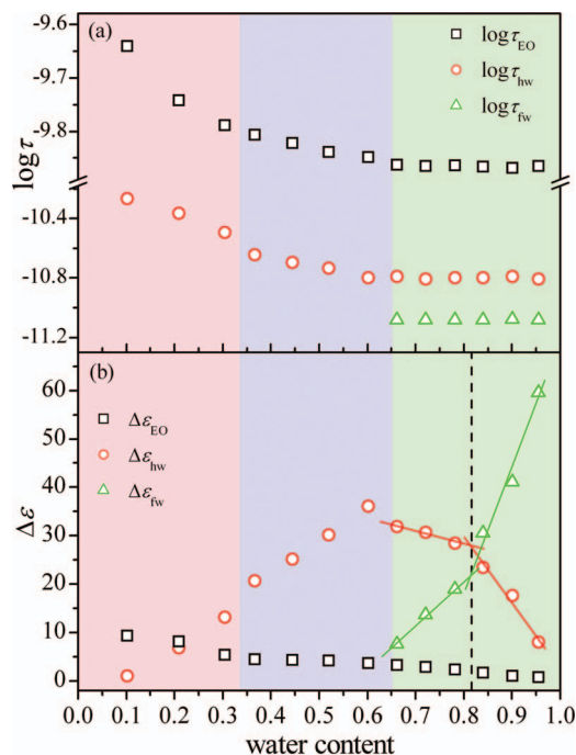
FIG. 6. Water content dependence of (a) the relaxation time and (b) the dielectric increment of the EO unit relaxation (open squares), hydration water relaxation (open circles), and free water relaxation (open triangles). The areas filled with different color represent different phase regions. The dashed line shows the inflexion point, and the solid lines are used for guiding the eyes.
