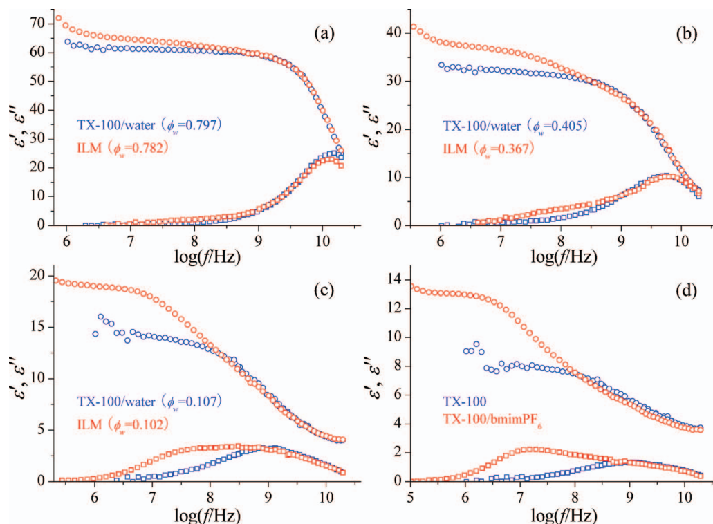
FIG. 3. (a), (b), and (c) The dielectric behaviors of ILMs and TX-100/water mixtures with comparable weight ratio between water and TX-100. (d) The dielectric behaviors of TX-100 and TX-100/bmimPF 6 mixture.
