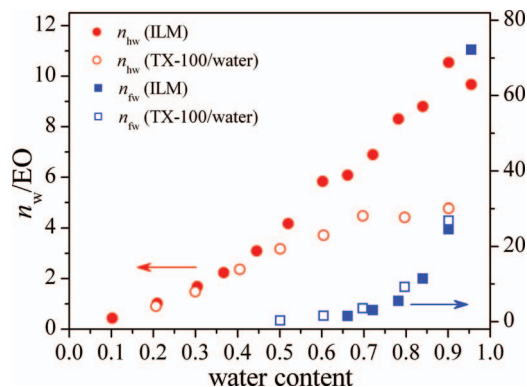
FIG. 7. Water content dependence of the number of water molecules per EO unit for ILMs (filled symbols) and TX-100/water mixtures (open symbols). The circles and squares represent the cases of hydration water and free water, respectively.
