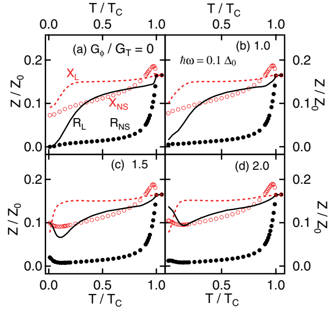
FIG. 4. (Color online) Impedance is plotted as a function of temperature for R_d/R_b = 0.2 and \hbar\omega = 0.1\Delta_0 . The length of the normal metal is fixed at L/\xi_{TC} = 1 . The symbols ( R_{NS} and X_{NS} ) represent the results of impedance for the whole NS bilayer in Eq. (16). The lines ( R_L and X_L ) are the local impedance at the surface of the normal metal given in Eq. (15).
