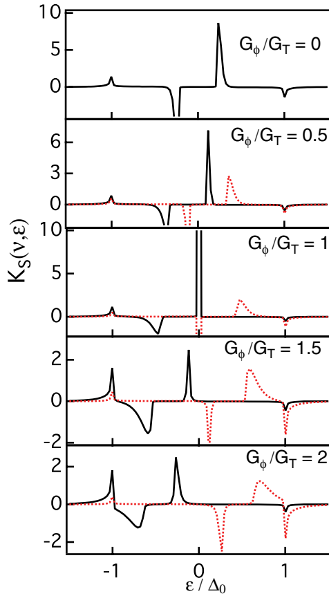
FIG. 3. (Color online) K_s function at the surface of the normal metal. The local pair density is calculated from Eq. (24). The results of K_s(\nu = 1, \epsilon) and K_s(\nu = -1, \epsilon) are shown with the solid and broken lines, respectively.
