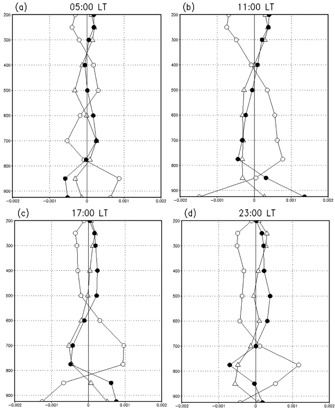
FIG. 9. Vertical distributions of composites of terms in the thermodynamic equation averaged over the Thar Desert ( 25^{\circ} – 30^{\circ} N, 67.5^{\circ} – 72.5^{\circ} E) at (a) 0000 UTC (0500 LT), (b) 0600 UTC (1100 LT), (c) 1200 UTC (1700 LT), and (d) 1800 UTC (2300 LT). Triangles denote horizontal advection, open circles denote vertical advection, and closed circles denote the residual, which includes diabatic heating ( \text{K s}^{-1} ).
