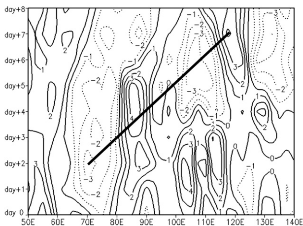
FIG. 4. Longitude–time diagram of the anomalous vorticity along 15°N at 850 hPa. Contours represent anomalous vorticity with a contour interval of 1 \times 10^{-6} \text{ s}^{-1} . Bold line represents the propagation path of the anomaly.
