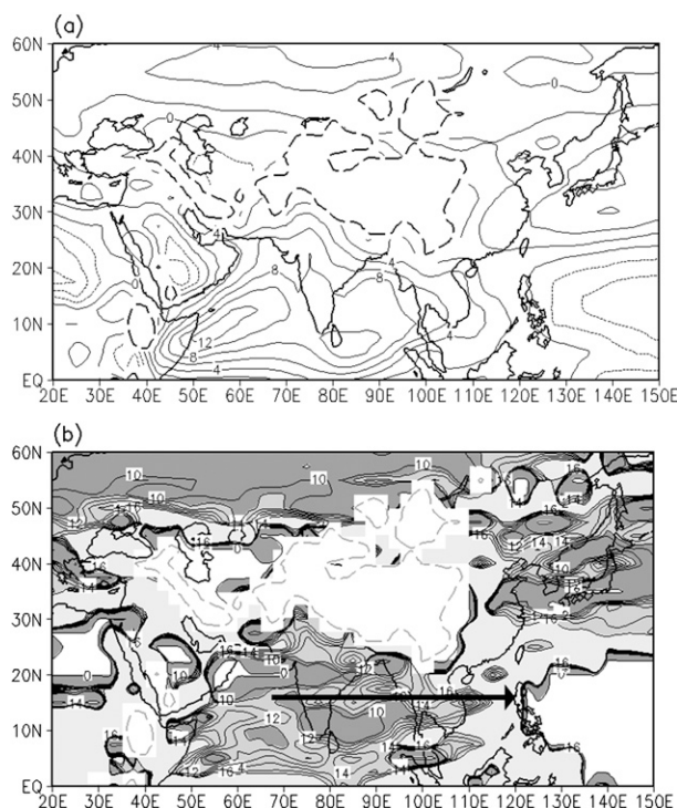
FIG. 5. (a) Average composite of the actual zonal wind velocity between day +2 and day +6 at 850 hPa. Contours represent the zonal wind speed with a contour interval of 2 \text{ m s}^{-1} . (b) The total stationary Rossby wavenumber was calculated from (a). Contours represent the wavenumber. Only values between 10 and 16 are drawn, with a contour interval of 1. Darker shading indicates smaller wavenumbers. No shading indicates areas where the stationary Rossby wave cannot exist. Thick line with an arrowhead shows the possible waveguide.
