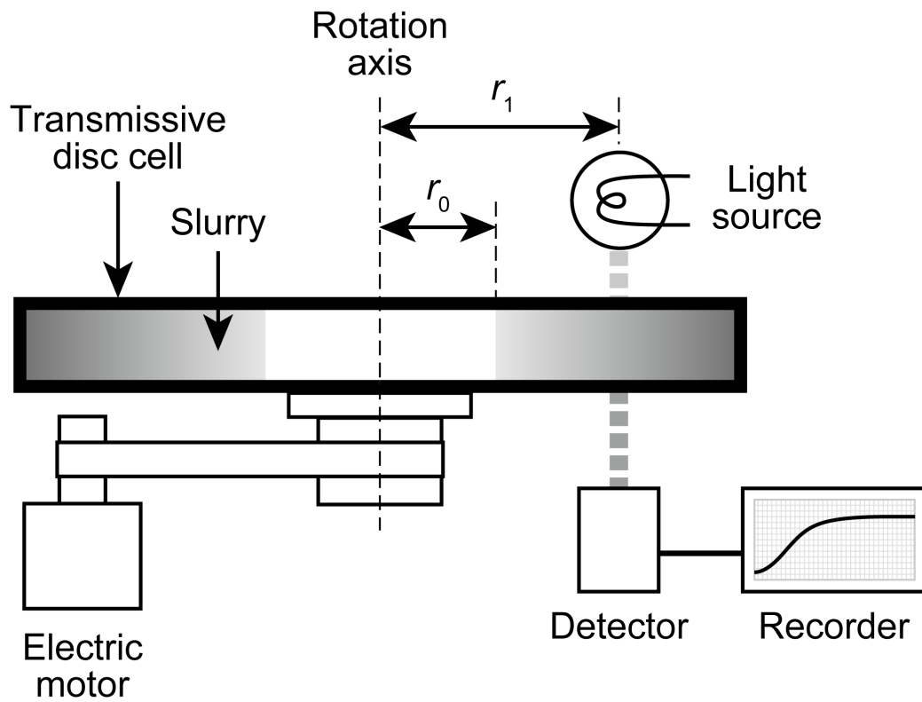
Fig. 4 Schematic diagram of the centrifugal type particle size analyzer.
