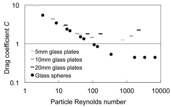
Fig. 13 Relationship between drag coefficient and particle Reynolds number in gravitational settling tests.
