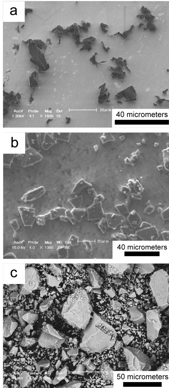
Fig. 1 Microphotographs of a) PTFE particles, b) glass flake particles, and c) quartz particles taken with scanning electron microscope.
