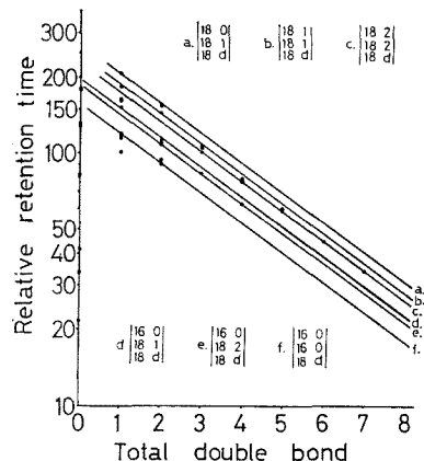
Fig. 2. Relation between relative retention time of triglyceride types and their total double bond.
