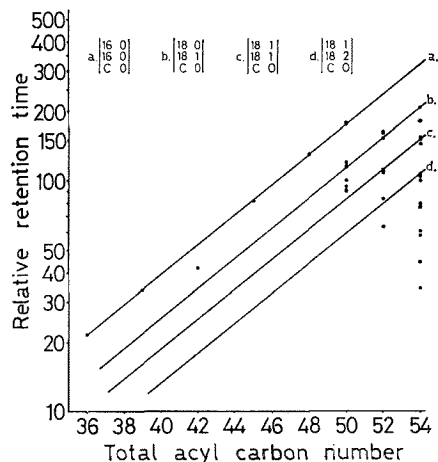
Fig. 1. Relation between relative retention time of triglyceride types and their total acyl carbon number.
