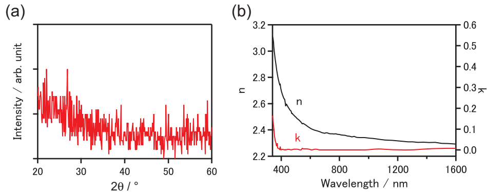
FIG. 2. (a) X-ray diffraction data and (b) refractive index for a non-patterned \text{TiO}_2/\text{SiO}_2/\text{Si} sample. Symbols of n and k indicate the refractive index and the extinction coefficient, respectively. The small peak and dip structures are artifacts caused by discontinuity of phase in the ellipsometric data.
