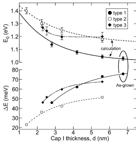
FIG. 5. The exciton ground-state energy E_0 (upper panel) and the intersub-level spacing \Delta E (lower panel) as a function of the cap I thickness. The cap I thickness of as-grown sample indicates average QDs height \sim 6.75 nm, which is estimated by the AFM image of a reference sample in Fig. 2(a). In the upper panel, the error bar indicates the FWHM of the exciton ground-state component for each sample. Note that cap I is a capping layer before IF step. The solid circles, open circles, and solid diamonds are for type 1, type 2, and type 3 samples, respectively.
