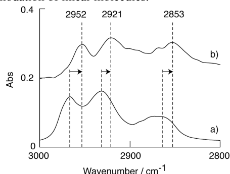
Figure 3. IR spectra (KBr pellet) of (a) heptane and (b) heptane trapped by C2-PW. For (b), the spectrum of C2-PW was subtracted from the raw spectrum.
