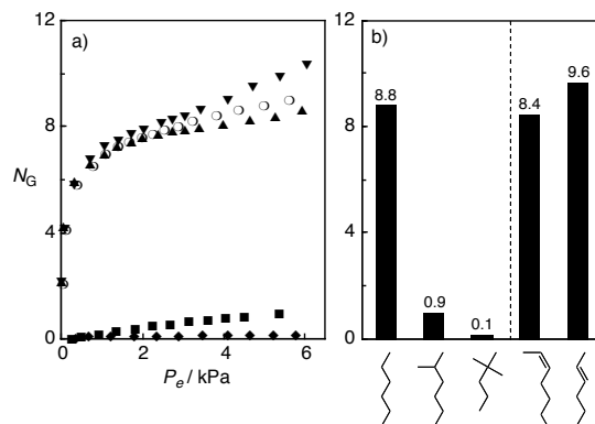
Figure 2. a) Sorption isotherms of heptane (○), 2-methylhexane (■), ( Z )-2-heptene (▲), ( E )-2-heptene (▼) (25 °C) and 2,2-dimethylpentane (◆) (20 °C) to C2-PW. Plots of the number of guest molecules trapped in a single unit cell ( N_G ) versus P_e . b) N_G at P_e = 5 kPa.
