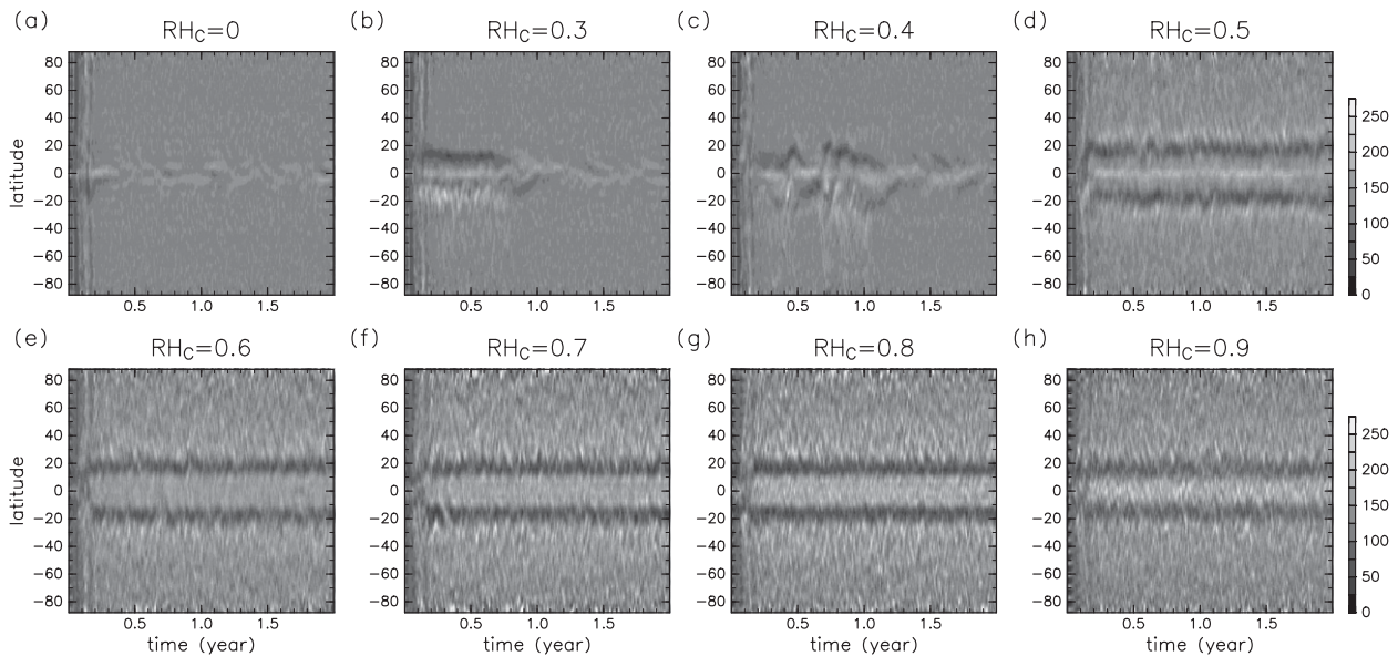
FIG. 1. Time-latitude sections of zonal mean precipitation ( \text{W m}^{-2} ; expressed in terms of latent heating) for the first 2 yr of the Cntrl runs. The RH_C values are shown above the panels.
