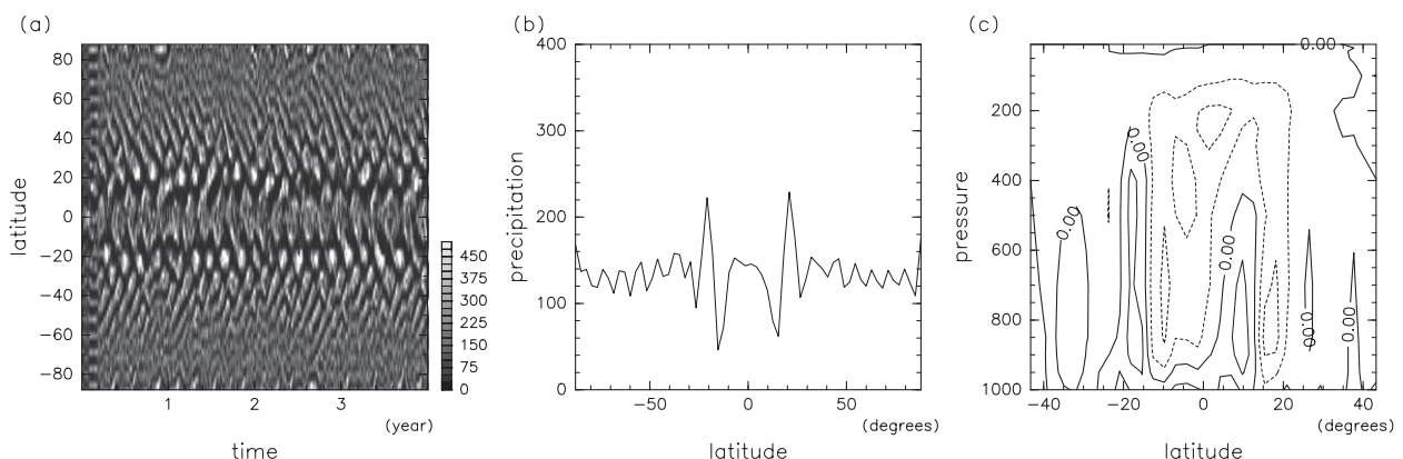
FIG. 10. As in Fig. 5, but for the Axsym run.
