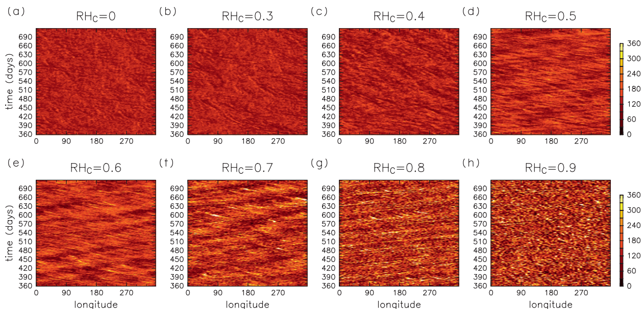
FIG. 6. Longitude–time plots of tropical precipitation averaged between 15°S and 15°N over the second model year of the Cntrl runs ( \text{W m}^{-2} ).
