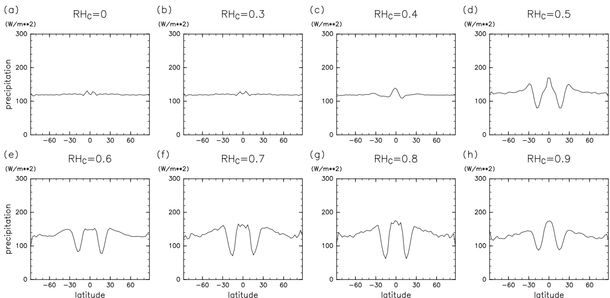
FIG. 2. Meridional distribution of zonal mean precipitation ( \text{W m}^{-2} ) averaged over the second model year of the Cntrl runs.
