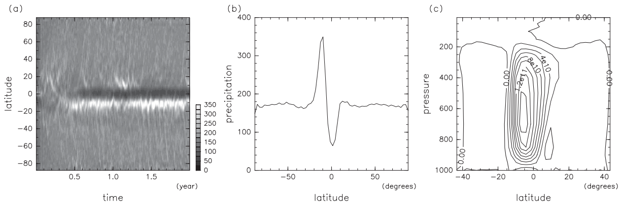
FIG. 5. Results from the run with RH_C = 0 in the 4-Col series: (a),(b) precipitation as in Figs. 1 and 2, respectively; (c) mass streamfunction \Psi ( \text{kg s}^{-1} ).
