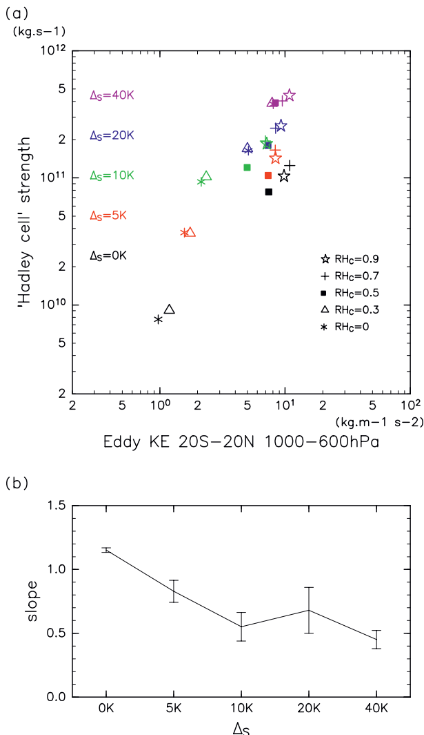
FIG. 13. (a) As in Fig. 8, but for the Y2-eq series. The RH_C values are indicated by different symbols; \Delta_S values by colors. (b) Slope of the linear least squares fit for each \Delta_S value based on the log-log scaling in (a). Standard errors are shown by the error bars.
