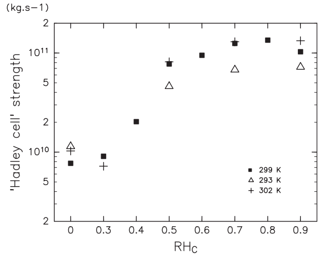
FIG. 4. Upward mass flux associated with the Hadley circulation \Delta \Psi_{600} (see below) in the Cntrl runs ( T_0 = 299 \text{ K} , filled squares) and the T0Chg runs ( T_0 = 293 and 302 \text{ K} , triangles and plus marks, respectively) averaged over the second model year. The abscissa is \text{RH}_C . The mass flux is defined as the difference between the maximum (in the Northern Hemisphere) and the minimum (in the Southern Hemisphere) of \Psi at 600 hPa in the tropics. Note that \text{RH}_C values supported in the T0Chg series are only 0, 0.3, 0.5, 0.7, and 0.9. Furthermore, the value for the run with T_0 = 293 \text{ K} and \text{RH}_C = 0.3 is not shown, since the resultant circulation is highly asymmetric (see text), so a comparison is meaningless.
