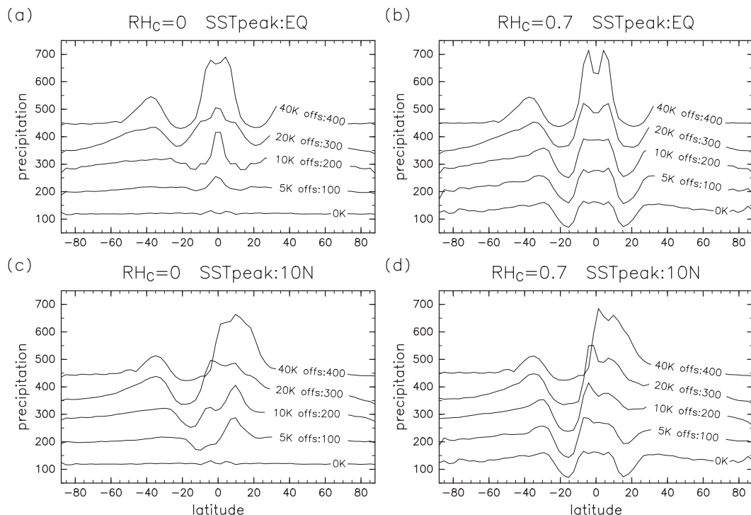
FIG. 12. Meridional distribution of precipitation averaged over the second model year in the (a),(b) Y2-eq and (c),(d) Y2-10N series when RH_C is (left) 0 and (right) 0.7. In each panel results for \Delta_S = 0, 5, 10, 20 , and 40 K are shown, with offsets of 0, 100, 200, 300, and 400 \text{ W m}^{-2} , respectively, for illustration purposes.
