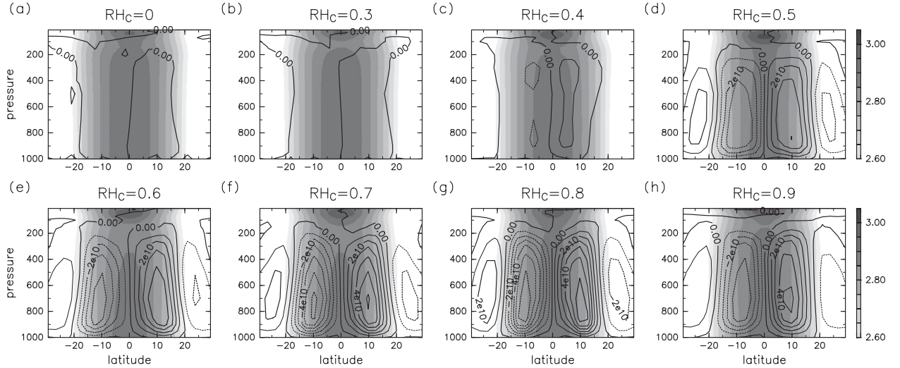
FIG. 3. Meridional mass streamfunction \Psi (contours; contour interval = 2 \times 10^{10} \text{ kg s}^{-1} ) and the absolute angular momentum \bar{m} (shading; interval = 0.05 \times 10^9 \text{ m}^2 \text{ s}^{-1} ) averaged over the second model year of the Cntrl runs.
