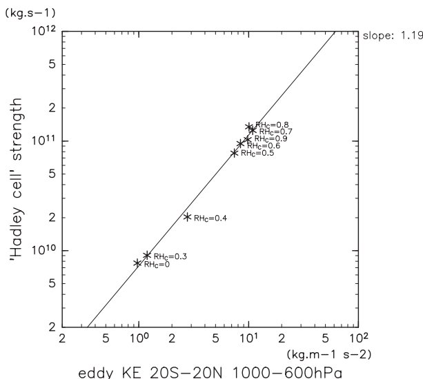
FIG. 8. Relation between the lower-tropospheric perturbation kinetic energy (kinetic energy of the deviation from the zonal mean horizontal winds averaged between 20^\circ\text{S} and 20^\circ\text{N} and 600 \leq p \leq 1000 hPa) and the upward mass flux of the Hadley circulation \Delta\Psi_{600} for the Cntrl series. The line shows the least squares fit.
