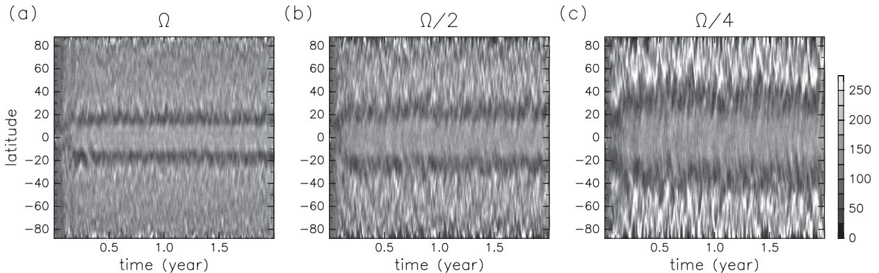
FIG. 11. As in Fig. 1, but for the RotChg series.
