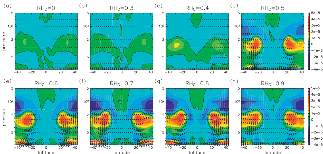
FIG. 15. The EP flux \mathbf{F} (arrows) and \rho_0^{-1} \nabla \cdot \mathbf{F} (shading) averaged over the second model year of the Cntrl runs. The divergence is multiplied by a constant factor to make the units in \text{m s}^{-2} . Unlike the other figures, the ordinate p is shown with a logarithmic scaling. The contour is plotted where the value is zero.
