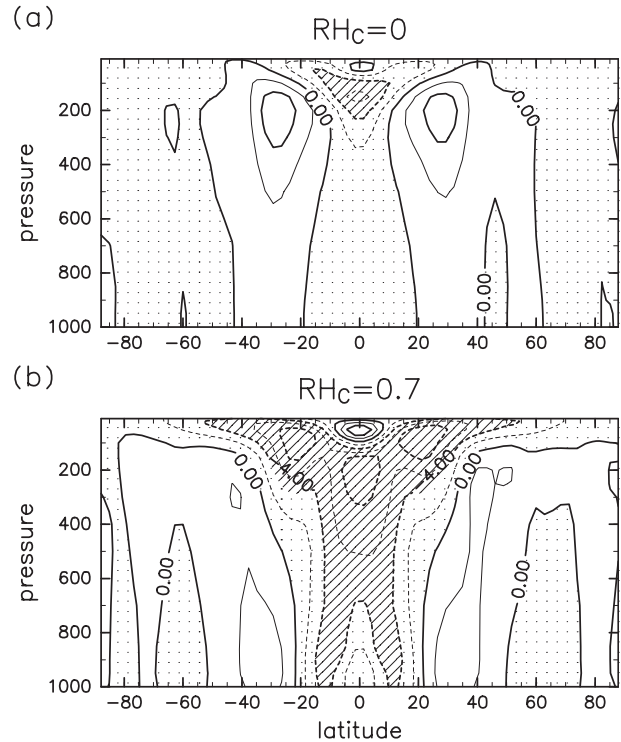
FIG. 14. Mean zonal wind averaged over the second model year in the Cntrl runs with RH_C = (a) 0 and (b) 0.7. Contour interval = 2 \text{ m s}^{-1} . Negative values are shaded.
