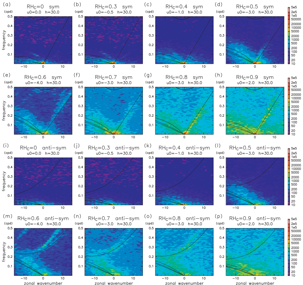
FIG. 7. Zonal wavenumber–frequency spectra of tropical precipitation averaged between 20°S and 20°N derived from the second model year of the Cntrl runs: spectra of (a)–(h) equatorially symmetric and (i)–(p) antisymmetric mode components. Note that coloring is made with a logarithmic scaling. Lines show the dispersion relation of equatorial waves with the equivalent depth h = 30 m subject to Doppler shifting with the background zonal velocity at the equator shown above each panel (by “ u_0 = ” \text{m s}^{-1} ). The values of the background velocity are determined subjectively from mean zonal wind in the equatorial lower troposphere.
