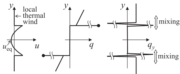
FIG. 16. Schematic illustration of how the baroclinic/barotropic instability occurs in the upper troposphere: u and q represent zonal mean zonal wind and potential vorticity, respectively; u_{\text{eq}} is the zonal wind at the equator. See text for the mechanism explanation.
