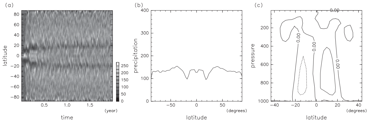
FIG. 9. As in Fig. 5, but for the Eqdmp run.
