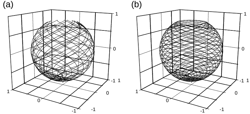
Fig. 2: Time evolution of the qubit.
