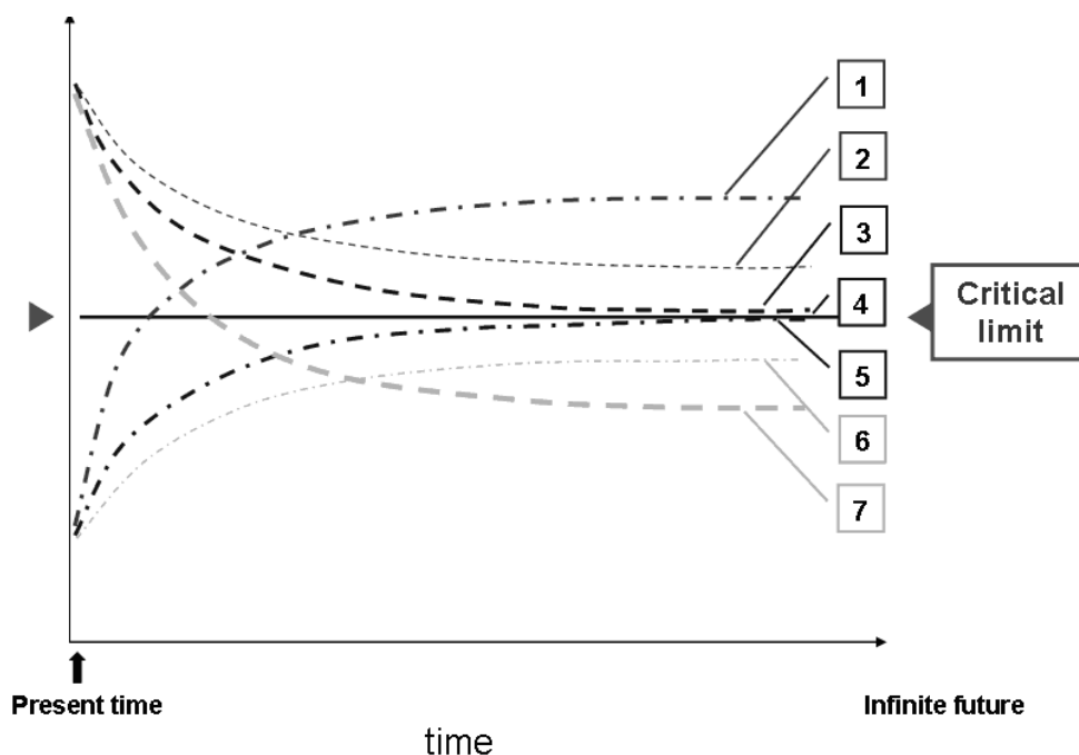
Fig. 3. Expected development of metal concentrations in environmental media in comparison to critical limits for different environmental situations (after Posch et al. 2003) Environmental situations:
