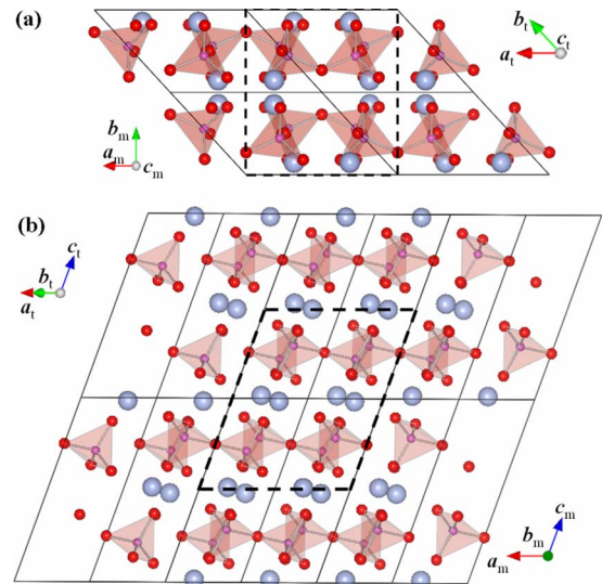
FIG. 1. (Color online) Crystal structure of monoclinic \beta - \text{Cu}_2\text{V}_2\text{O}_7 depicted with optimized crystallographic parameters. Views projected onto (a) (001) and (b) (010) planes. Gray (large), pink (small), and red (dark) spheres denote the Cu, V, and O atoms, respectively. Thick dashed lines denote the monoclinic C2/c unit cell. Eight primitive unit cells ( 2a_1 \times 2b_1 \times 2c_1 , space-group P1 ) are drawn with thin solid lines. Axes a_m , b_m , and c_m denote the directions of lattice vectors of the monoclinic cell. Axes a_t , b_t , and c_t denote the directions of lattice vectors of the triclinic primitive cell.
