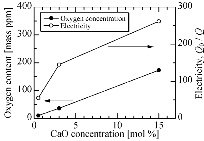
Figure 6. Oxygen concentration and charged electricity.
