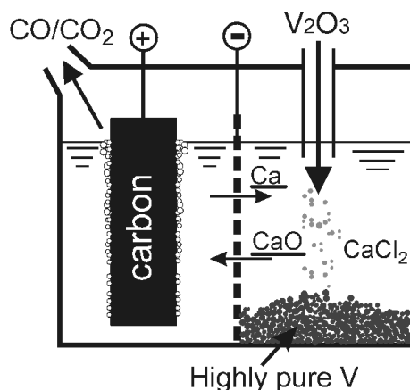
Figure 1. Concept of OS process for V production.
