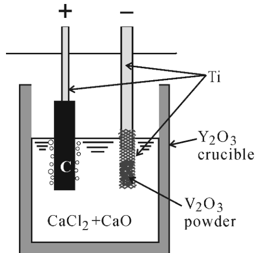
Fig. 3 Experimental arrangement.
