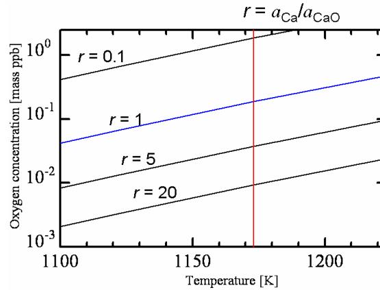
Figure 2. Oxygen concentration in \alpha -V as a function of temperature.
