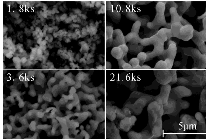
Figure 5. SEM images of the obtained V particles.
