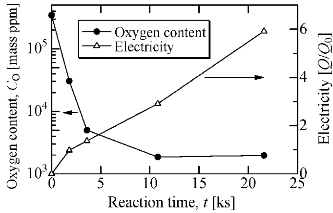
Figure 4. Oxygen concentration in the obtained powders.
