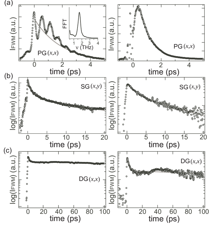
Figure 1: Typical signals of two-pulse and three-pulse FWM measurements in 120-Å SQW (left column) and 48-Å SQW (right column) at 10 K. (a) Phase relaxation of excitons monitoring the decay of polarization grating (PG) by two-pulse FWM. inset (left column): Fourier transformed spectrum of the signal. The peak due to the quantum beat is found to be \sim 1.64 THz (6.8 meV). (b) Exciton Spin relaxation monitoring the decay of spin density grating (SG) by three-pulse FWM. (c) Exciton lifetime monitoring the decay of exciton density grating (DG) by three-pulse FWM. In (a) of the right column, the spiky signal around the time origin is due to interference of two pulses and has no influence to obtain the phase relaxation time.
