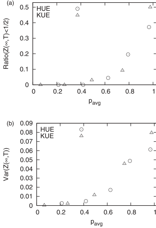
FIG. 4. (a) Ratios of the suboptimal [Z(\infty, T) < 1/2] cases, which are given in the last column of Table III, and (b) the variance \text{Var}(Z(\infty, T)) are plotted vs p . The symbols \circ and \triangle indicate the results of HUE and KUE, respectively.
