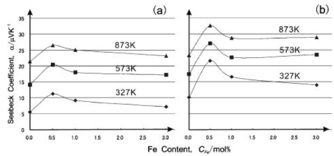
Fig. 7 Dependency of the Seebeck coefficient on Fe addition. (a): (\text{Co} + \text{Fe})\text{:Al:C} = 3.0:1:0.56 , (b): (\text{Co} + \text{Fe})\text{:Al:C} = 3.4:1:0.75 .
