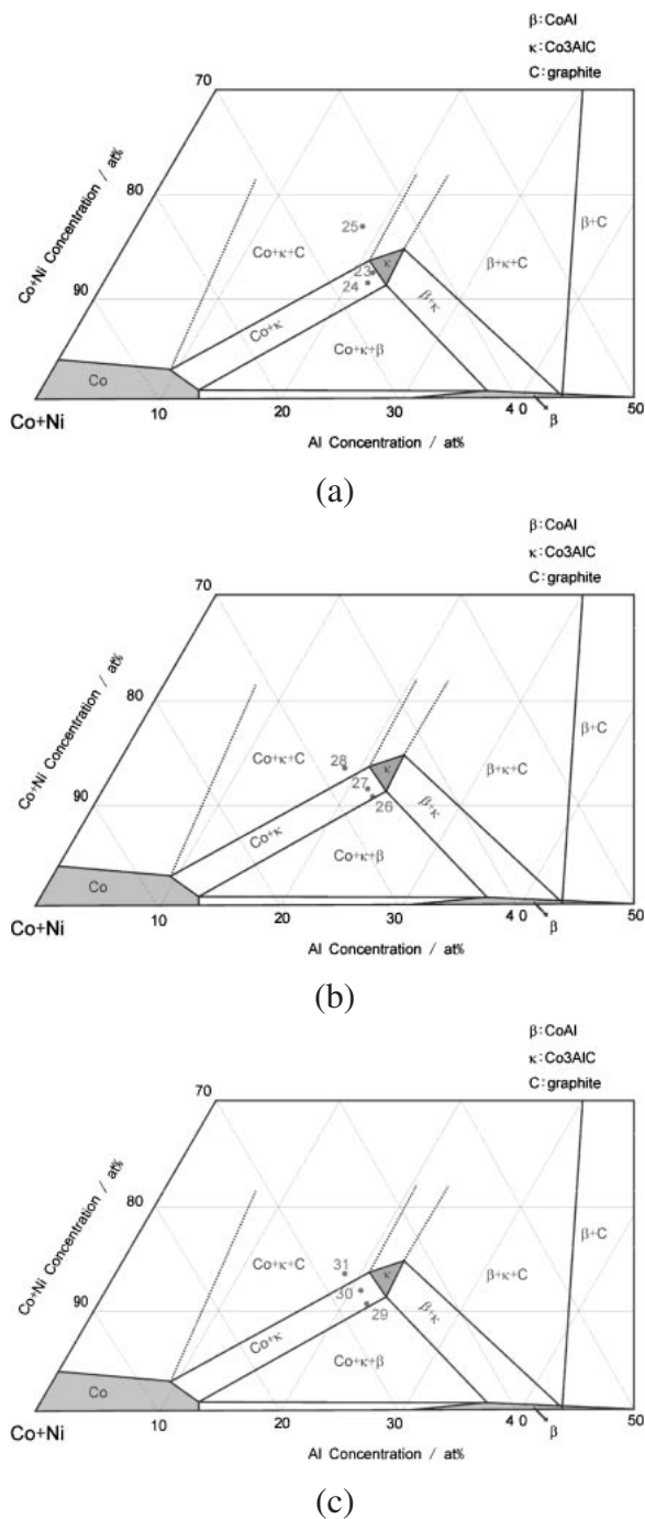
Fig. 8 Phase equilibria in the vicinity of the \kappa phase in the Co-Ni-Al-C quaternary system. (a) 0.5 mol% Ni addition, (b) 1.0 mol% Ni addition and (c) 3.0 mol% Ni addition.
