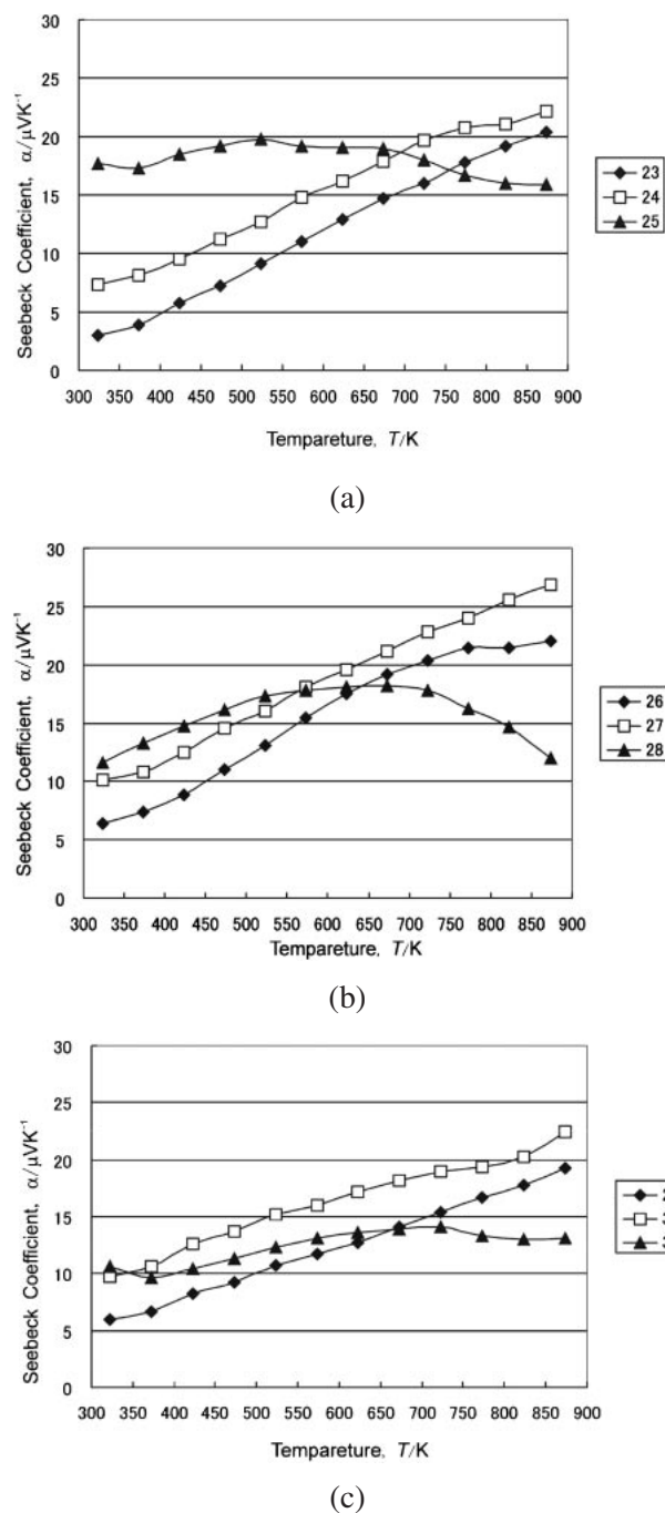
Fig. 9 Seebeck coefficient for the samples in which a part of the Co was replaced by 0.5 mol% Ni (a), 1.0 mol% Ni (b), and 3.0 mol% Ni (c).
