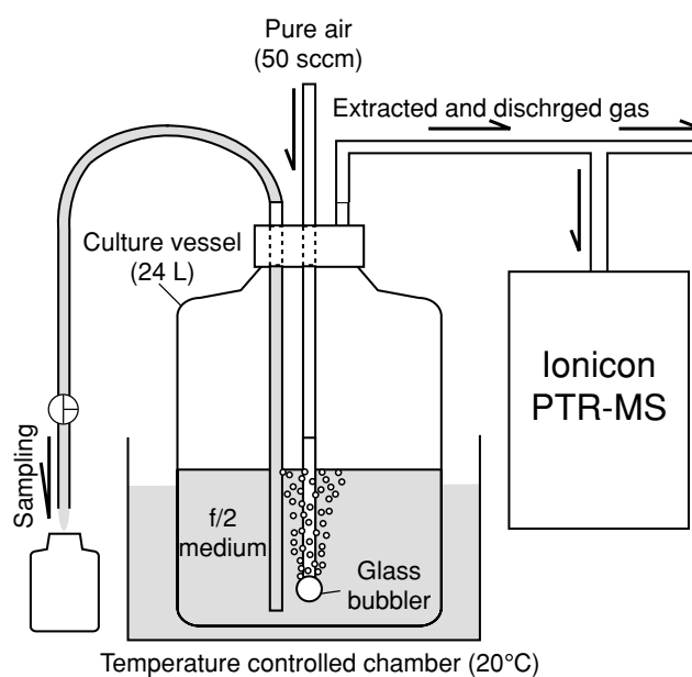
Fig. 1. Schematic diagram of the culture experiment and measurement system.
