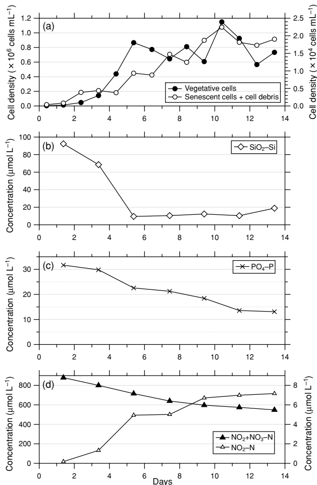
Fig. 2. Time course of (a) cell density of vegetative cells (left axis) and senescent cells plus cell debris (right axis), and concentrations of (b) silicate, (c) phosphate, and (d) nitrite plus nitrate (left axis) and nitrite (right axis) during the culture period.
