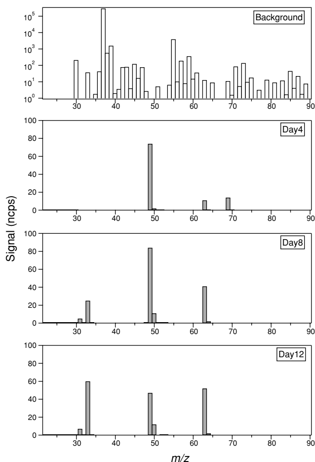
Fig. 3. Mass spectra for background and sample measurements. The mass spectra for the sample measurements were at 0 o'clock on days 4, 8, and 12. The background signals were subtracted for the sample mass spectra.
