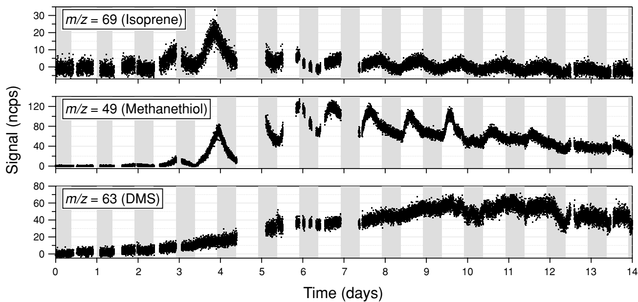
Fig. 4. Time series of PTR-MS signals at m/z 69, 49, and 63. Shaded areas indicate dark periods. Time-zero corresponds approximately to 30 h after inoculation to allow time for purging of possible gas contaminants.
