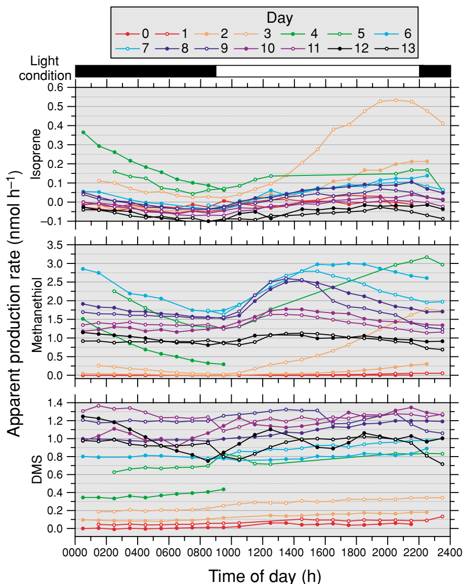
Fig. 5. Diurnal variation in apparent production rates of isoprene ( m/z 69), methanethiol ( m/z 49), and DMS ( m/z 63). The data are averages for each hour. A color version of this figure is available online.
