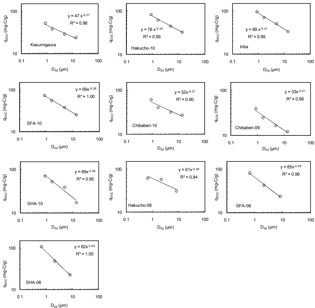
Figure S5. Plots of q_{DOC} as a function of median carbon diameter ( D_{50} ). Values of q_{DOC} were calculated for the carbon dose, at which 50% of the initial aqueous-phase DOC concentration (1.5 mg-C/L) was adsorbed.
