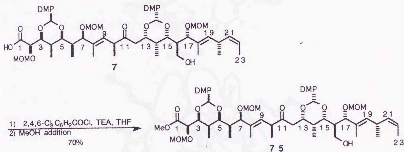
Scheme 27
