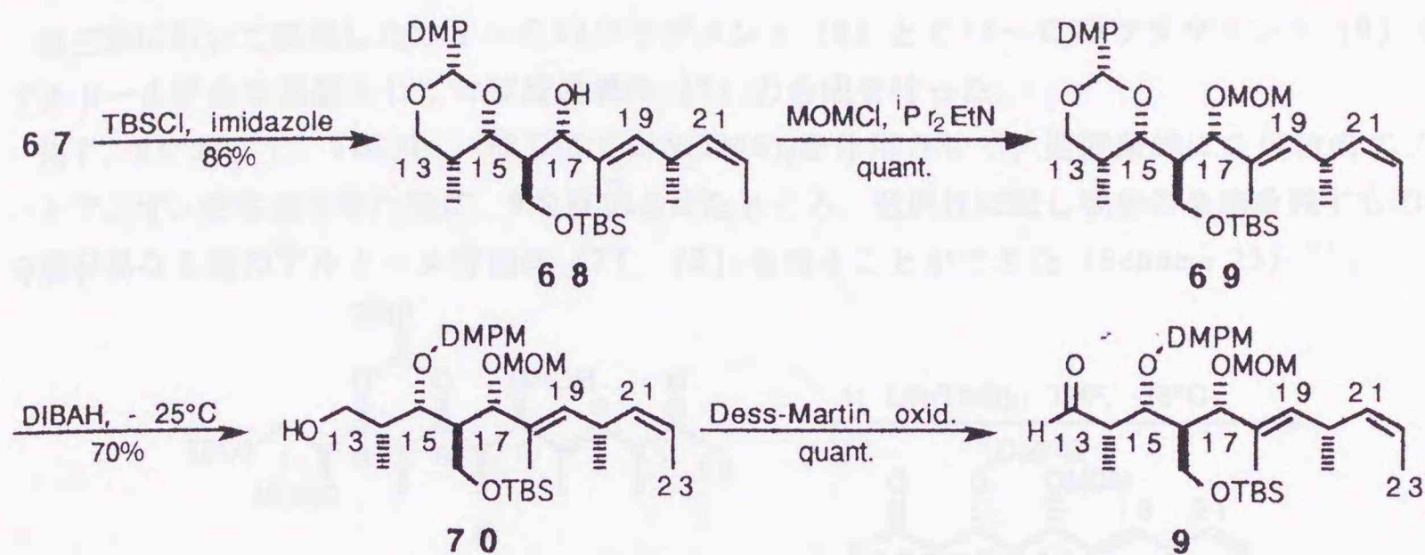
Scheme 22
