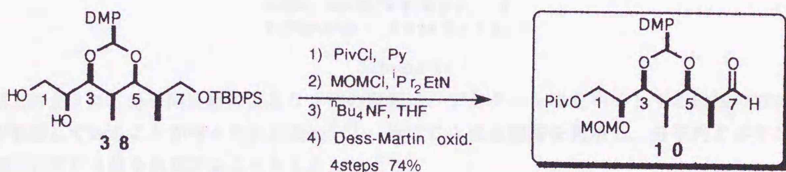
Scheme 10
