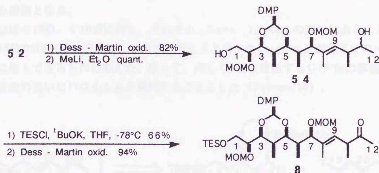
Scheme 15
