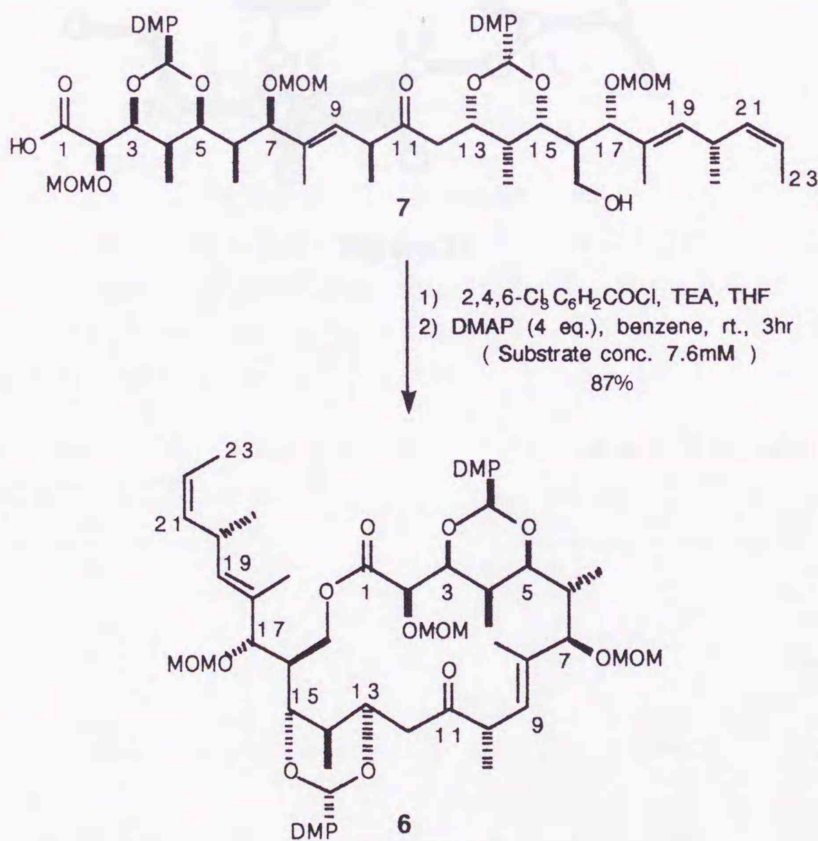
Scheme 26
