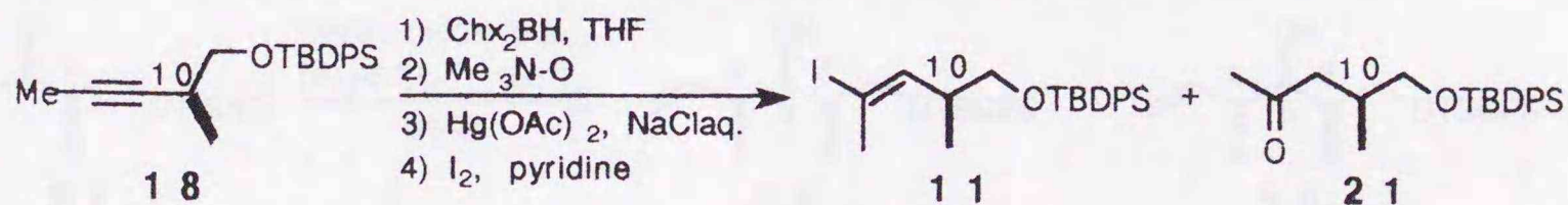
Scheme 4
