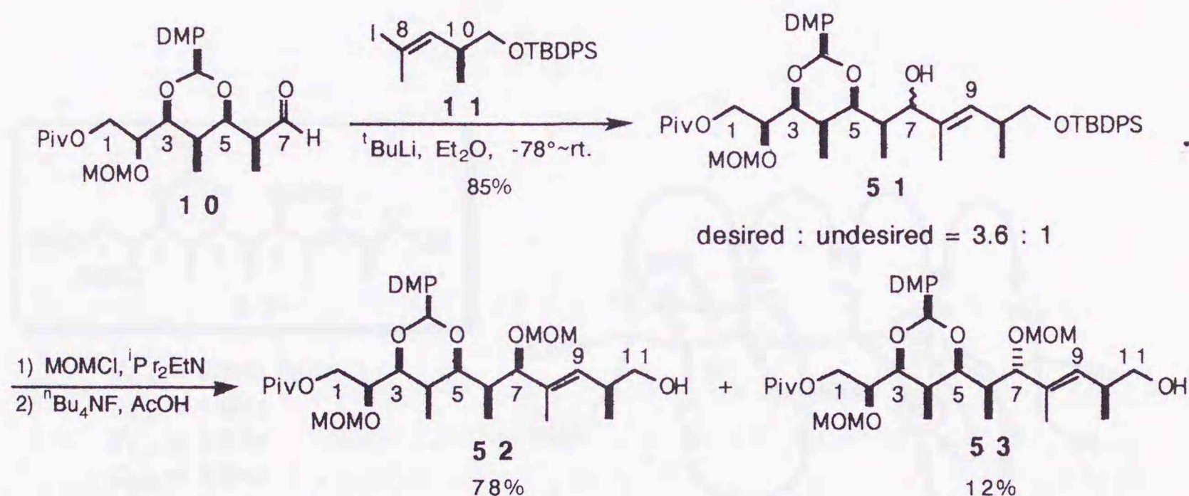
Scheme 14
