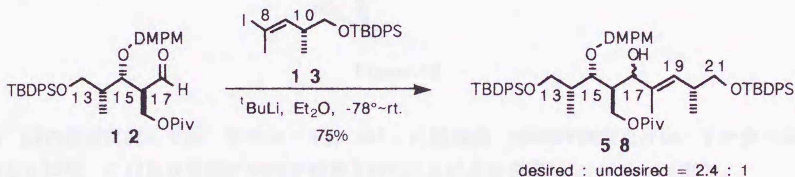
Scheme 18
