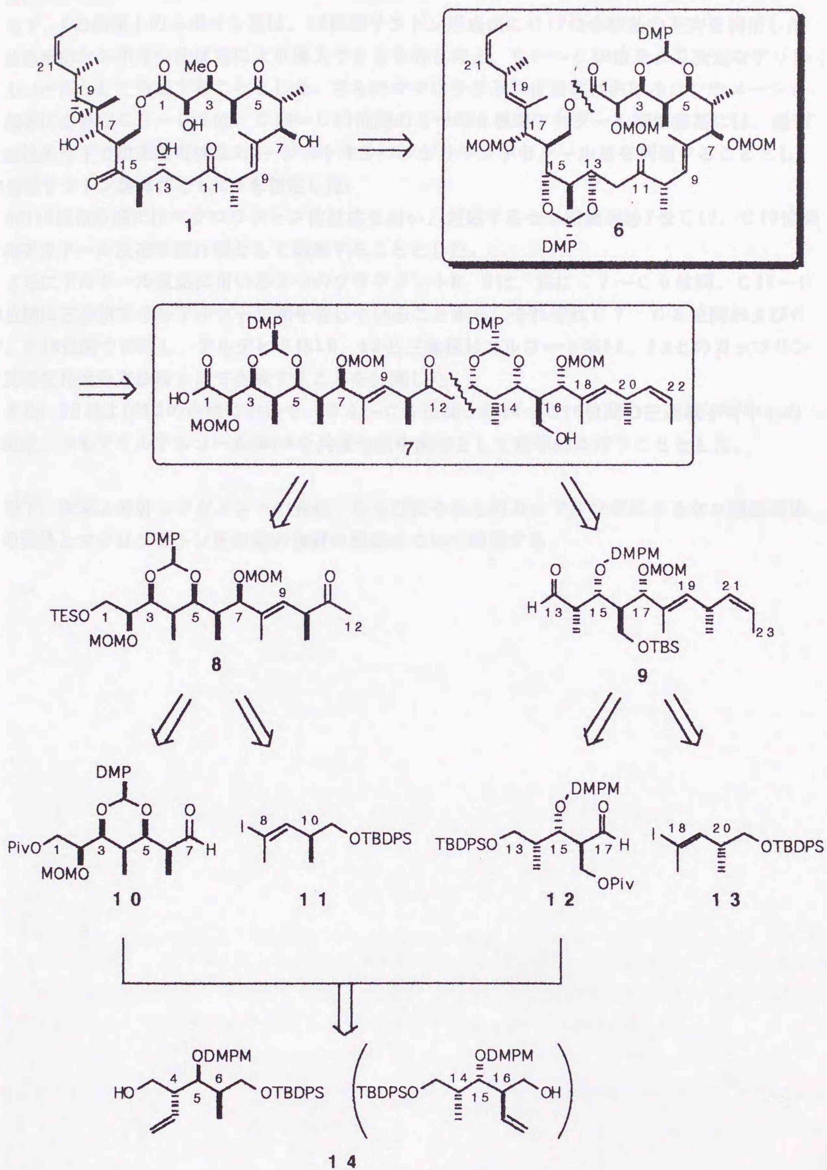
Scheme 2
