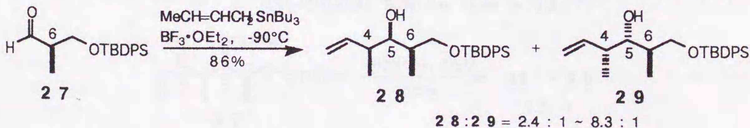
Scheme 6
