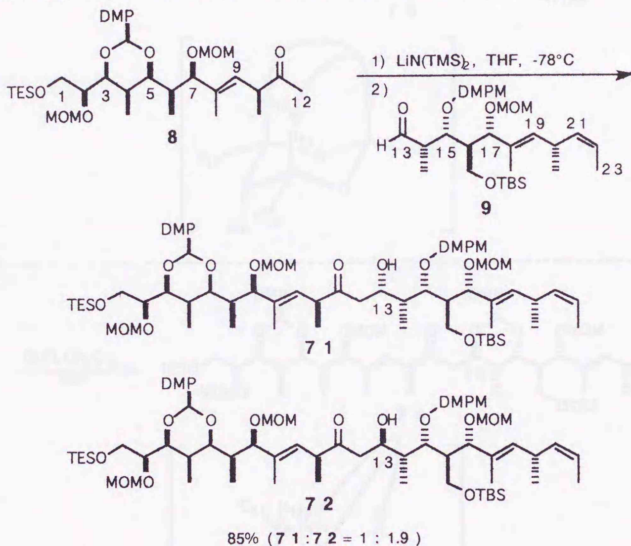
Scheme 23
