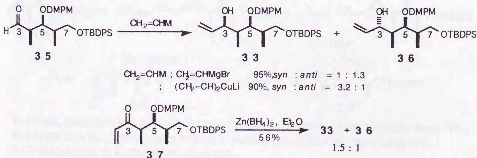
Scheme 8
