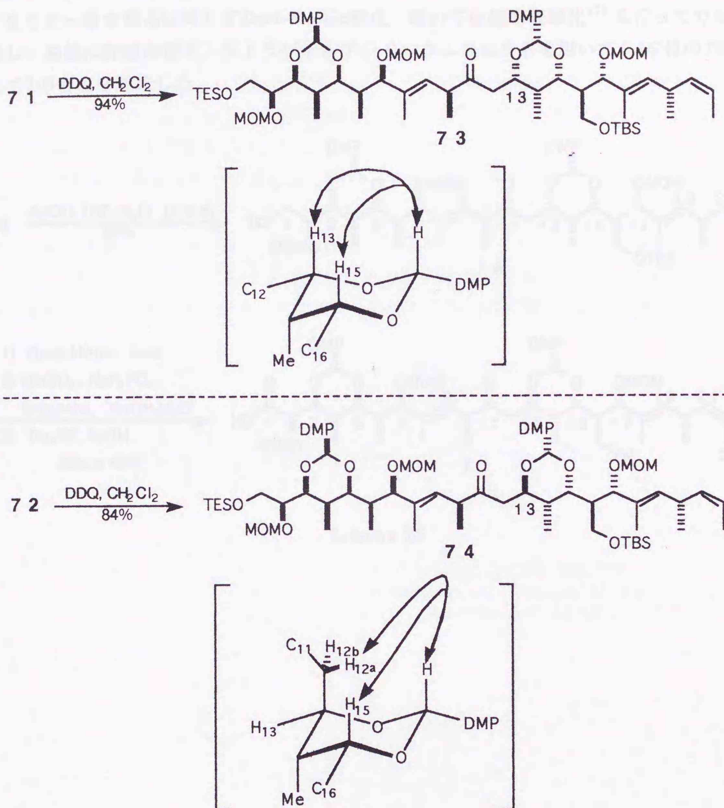
Scheme 24
