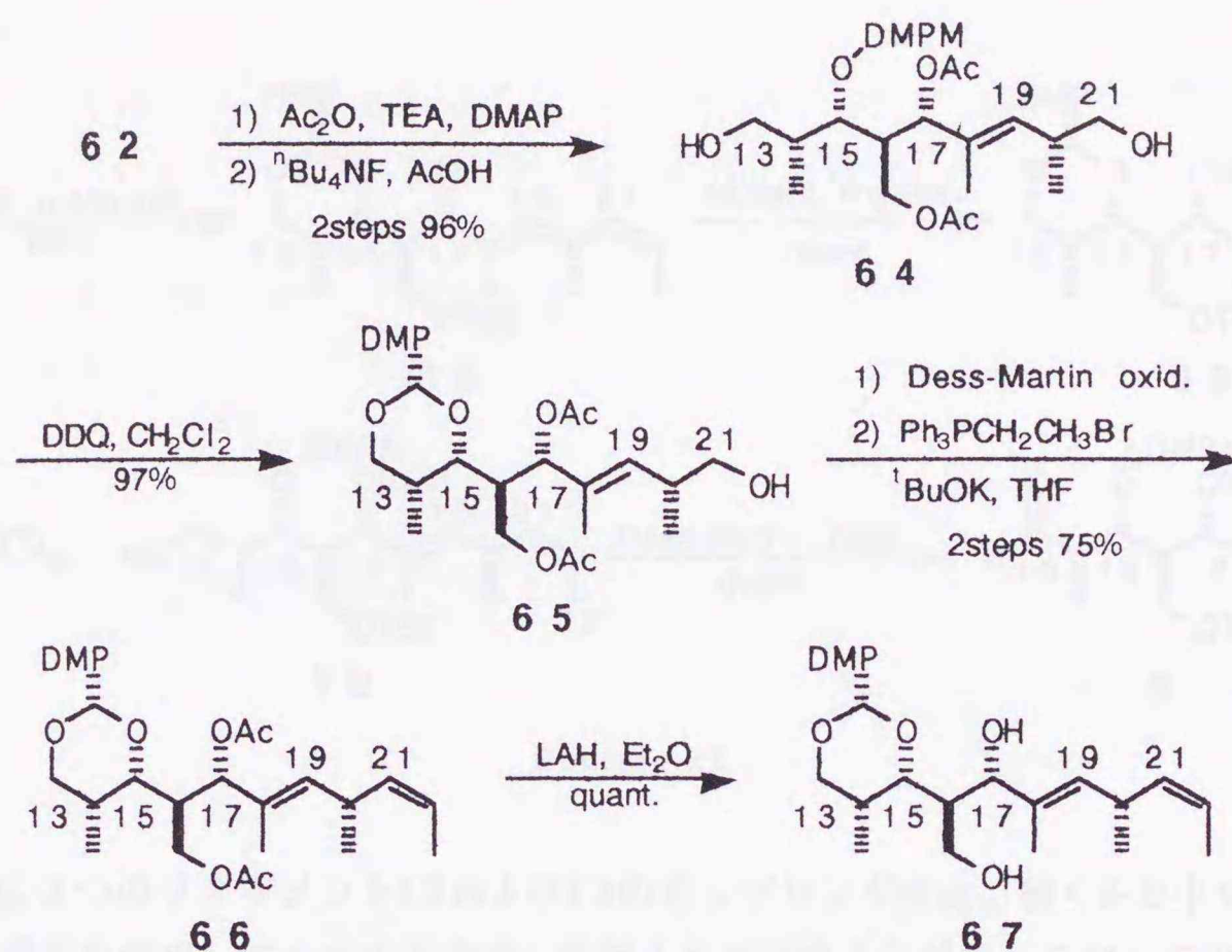
Scheme 21
