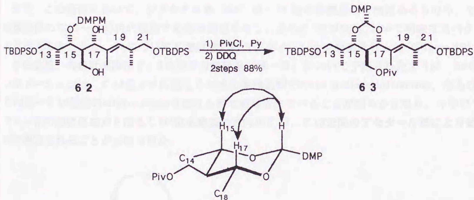
Scheme 20
