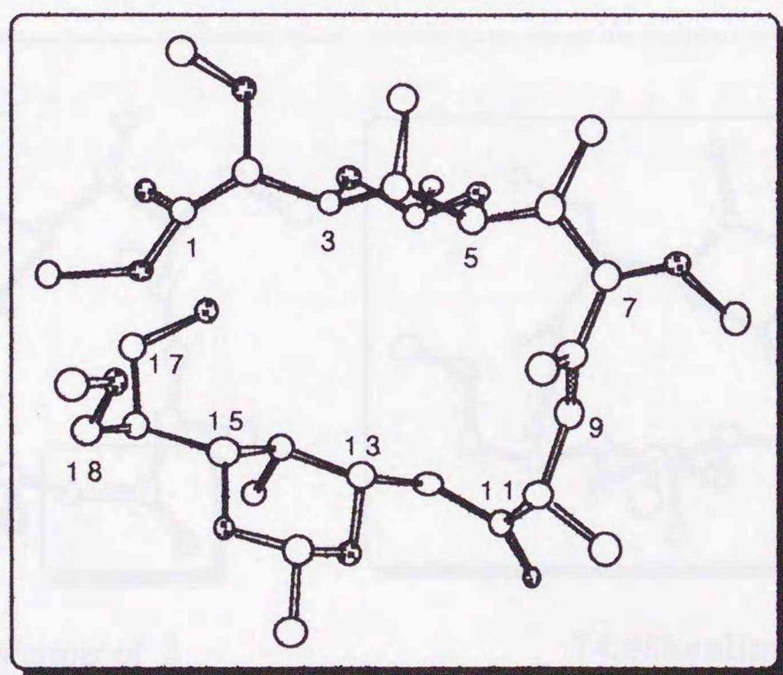
Starting geometry ( 3-2 )
