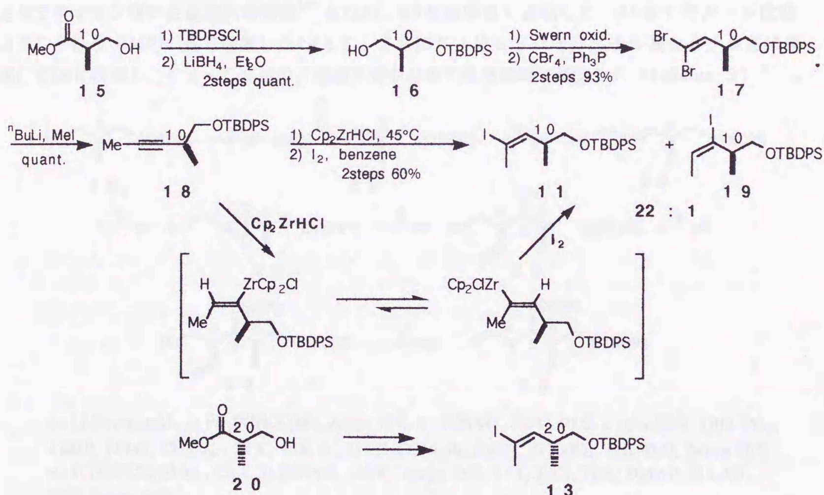
Scheme 3
