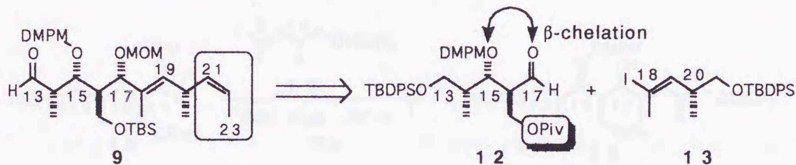
Scheme 16
