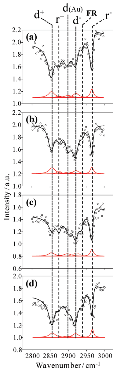
Figure 2. SFG spectra of (a) \equiv\text{Si}-(\text{CH}_2)_9\text{CH}_3 (C10), (b) \equiv\text{Si}-(\text{CH}_2)_{11}\text{CH}_3 (C12), (c) \equiv\text{Si}-(\text{CH}_2)_{13}\text{CH}_3 (C14), and (d) \equiv\text{Si}-(\text{CH}_2)_{17}\text{CH}_3 (C18) upon thermal evaporation of gold overlayers (10 nm thick). The solid lines (in black) show the best fits to the experimental data (open circles) based on eqs 1 and 2; the deconvoluted peaks are shown in red at the bottom (see main text for details).
