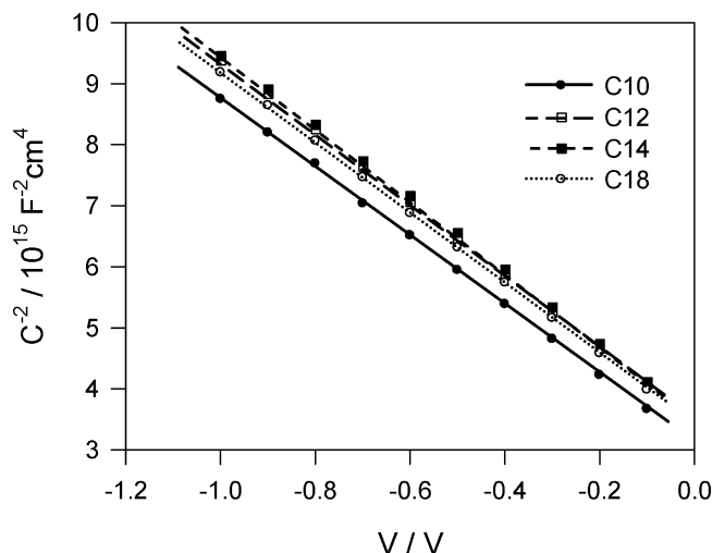
Figure 5. Mott–Schottky (M–S) plots of Au/alkyl monolayer/Si junctions; the gold contacts were prepared via thermal evaporation.
