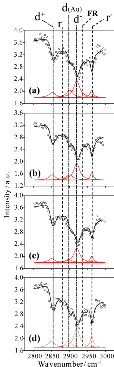
Figure 3. SFG spectra of (a) \equiv\text{Si}-(\text{CH}_2)_9\text{CH}_3 (C10), (b) \equiv\text{Si}-(\text{CH}_2)_{11}\text{CH}_3 (C12), (c) \equiv\text{Si}-(\text{CH}_2)_{13}\text{CH}_3 (C14), and (d) \equiv\text{Si}-(\text{CH}_2)_{17}\text{CH}_3 (C18) upon sputtering deposition of 10 nm thick gold overlayers. The solid lines (in black) show the best fits to the experimental data (open circles) based on eqs 1 and 2; the deconvoluted peaks are shown in red at the bottom (see the main text for details).
