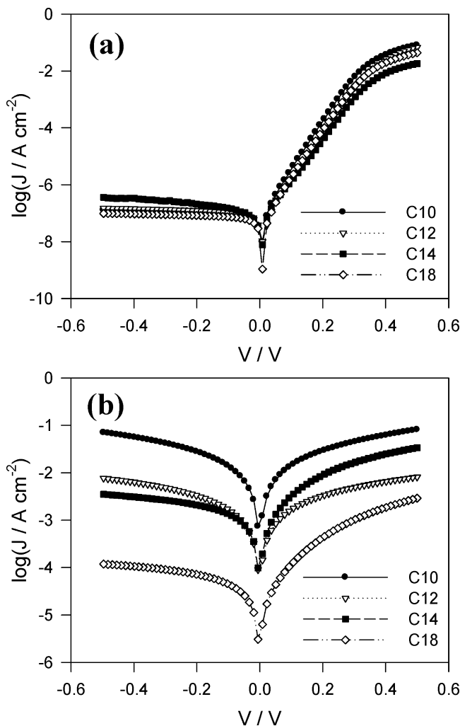
Figure 4. Current density–bias voltage ( J – V ) plots of Au/alkyl monolayer/Si junctions, for which the alkyl chain length was systematically varied. The gold contacts were prepared by (a) thermal evaporation and (b) sputtering deposition.
