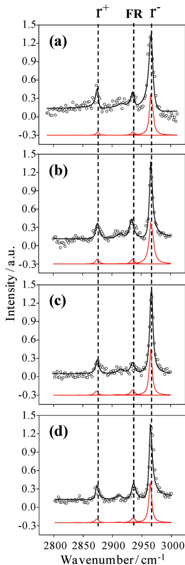
Figure 1. SFG spectra of (a) \equiv\text{Si}-(\text{CH}_2)_9\text{CH}_3 (C10), (b) \equiv\text{Si}-(\text{CH}_2)_{11}\text{CH}_3 (C12), (c) \equiv\text{Si}-(\text{CH}_2)_{13}\text{CH}_3 (C14), and (d) \equiv\text{Si}-(\text{CH}_2)_{17}\text{CH}_3 (C18). The solid lines (in black) show the best fits to the experimental data (open circles) shown in eqs 1 and 2; the deconvoluted peaks are shown in red at the bottom (see the main text for details).
