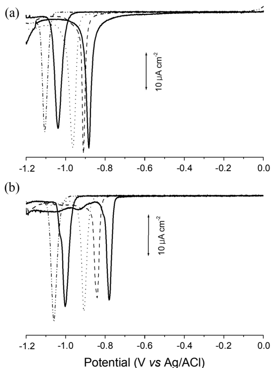
Figure 2. Linear sweep voltammograms of (a) 1, n -alkanedithiol ( n = 2, 4, 6, 8, 10) and (b) alkanethiol ( n = 2, 4, 6, 8, 10) SAM on a Au(111) electrode in 0.1 M KOH solution with potential scan rate of 20 mV s -1 .
