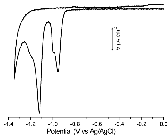
Figure 12. Cyclic voltammogram of a DT/Au/HDT on Au(111) electrode in 0.1 M KOH solution with a scan rate of 20 mV s -1 .
