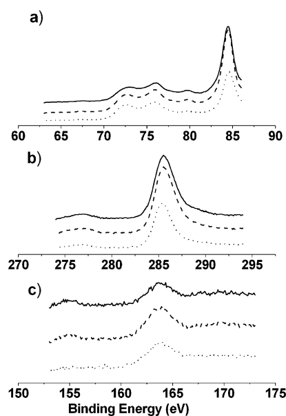
Figure 6. XP spectra of Pt/BDMT/Au electrodes with different exit angles ( 90^\circ : solid line, 60^\circ : dashed line, 30^\circ : dotted line) in the region of (a) Pt 4f with Au 4f_{7/2} peak, (b) C 1s, and (c) S 2p.
