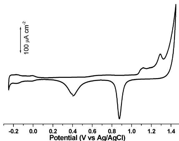
Figure 11. CV of a Pt-deposited BDMT SAM-modified Au(111) electrode, which was prepared in a 0.05 M \text{H}_2\text{SO}_4 solution containing \text{PtCl}_4^{2-} ions at +0.4 V, measured in 0.05 M \text{H}_2\text{SO}_4 solution with a scan rate of 20 \text{ mV s}^{-1} after the reductive desorption of the BDMT SAM in a 0.1 M KOH solution by scanning the potential to -1.30 V.
